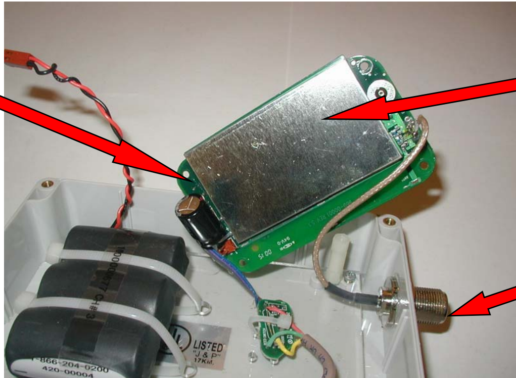
Figure 3 Solder Side View of Main Board (with RF Section Metal Shield Cover)
