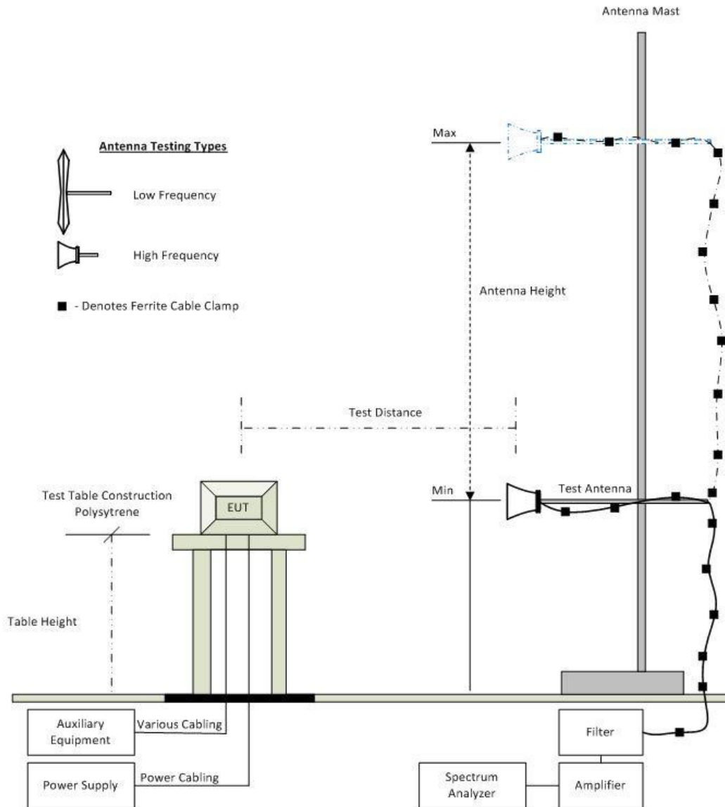
Radiated Emission Measurement Setup Pictorial Representation
