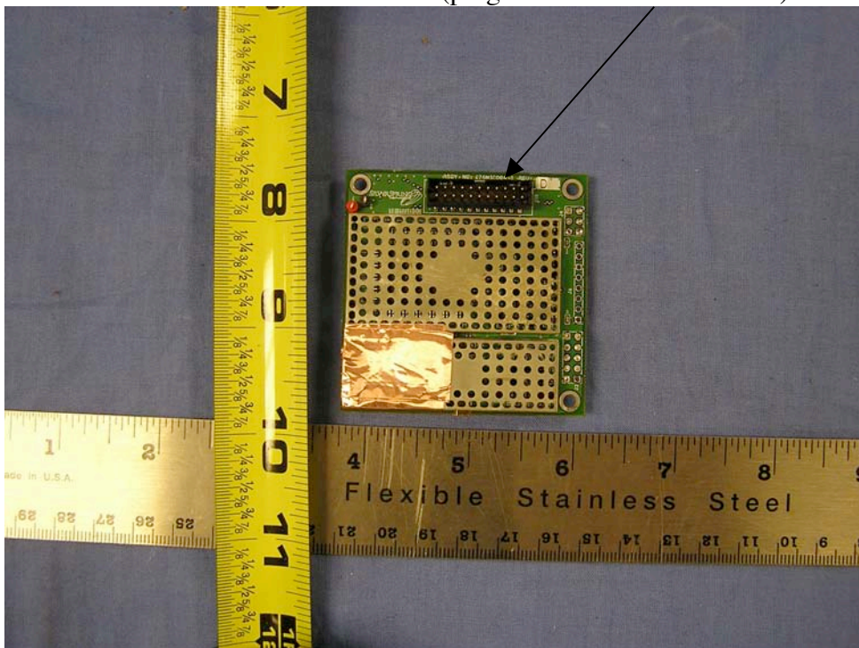
Bottom view radio board with shields (plug to meter interface board)
