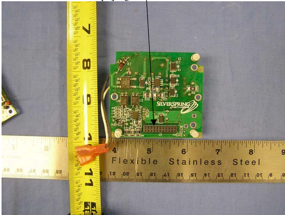
Meter interface board Top (plug for radio board)
