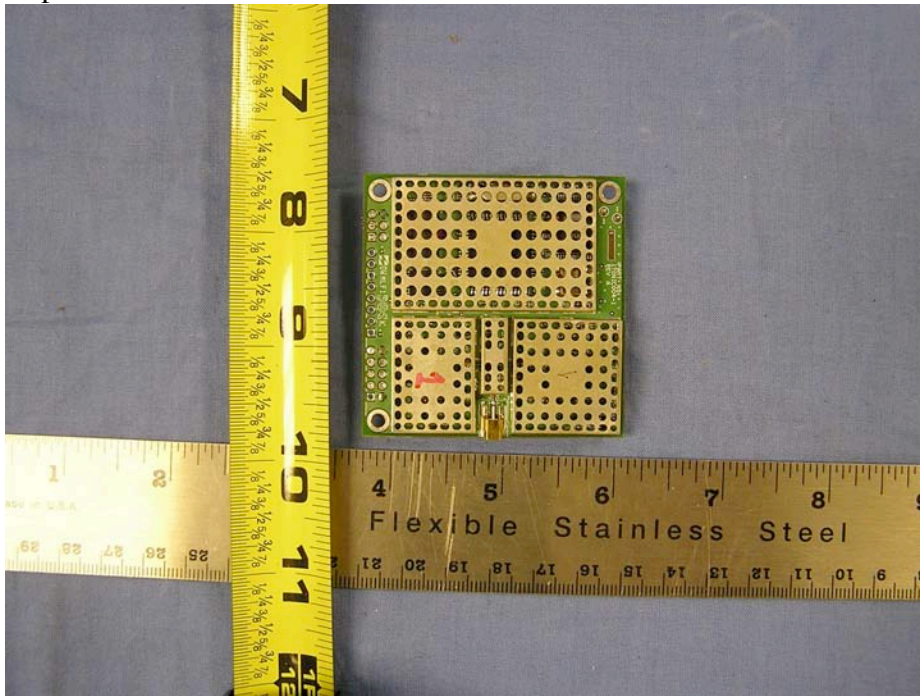
Top view Radio Board with shields
