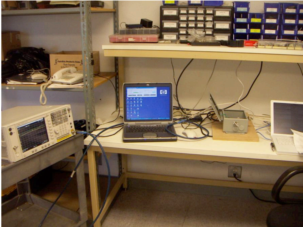
Antenna port conducted emissions test set-up
