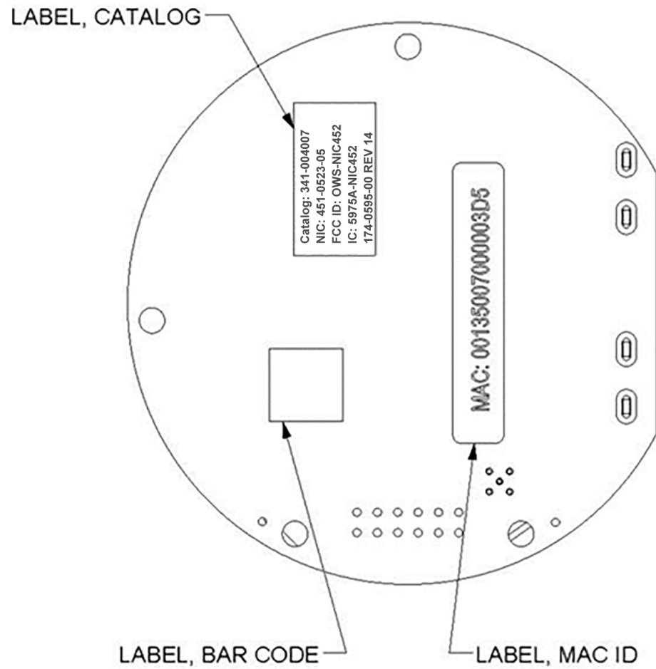
Figure 4. Label locations on the Silver Spring Street Light NIC
