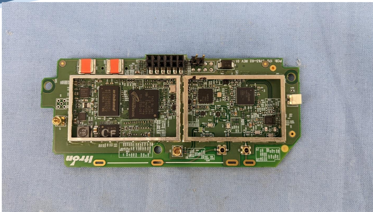
Top View Shields Removed
