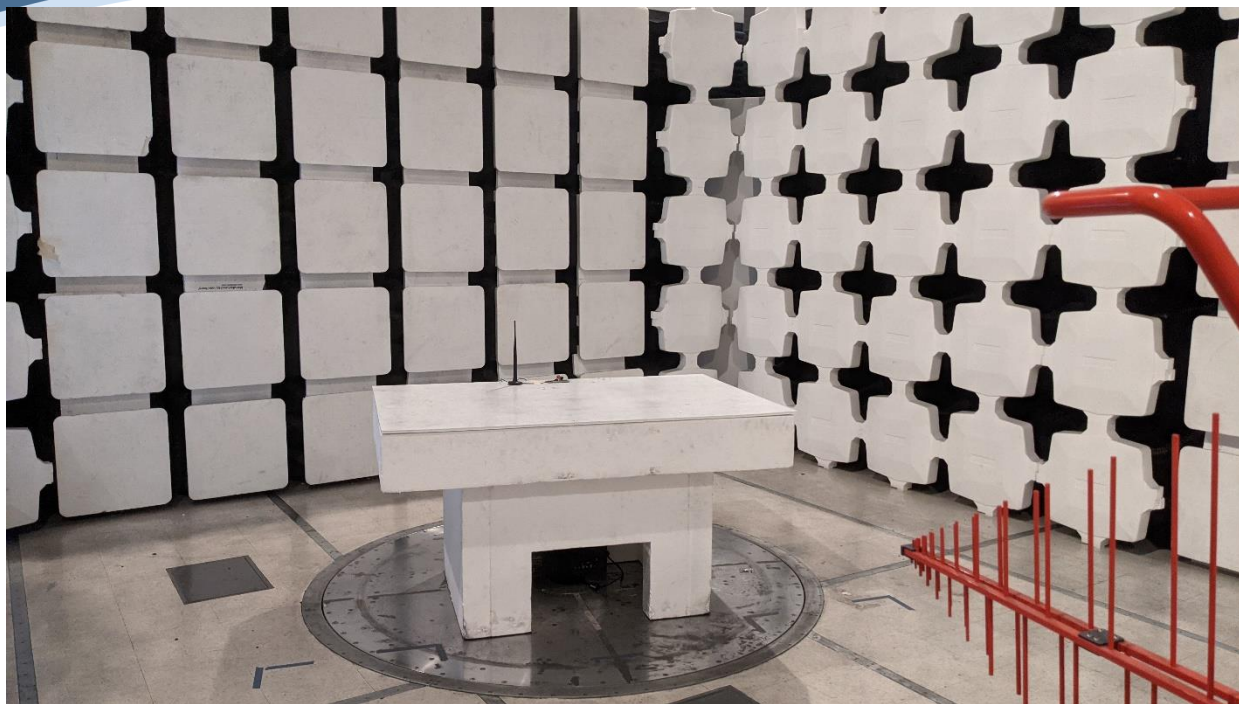
Digital Emissions Below 1GHz
