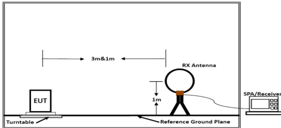
Below 30MHz
