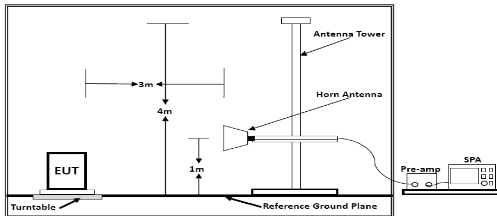
Above 1GHz
