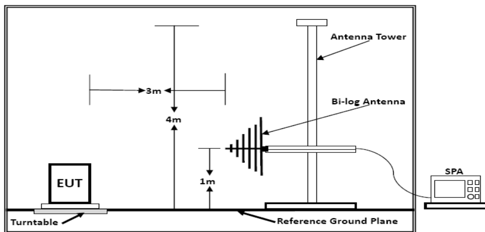
Below 1GHz
