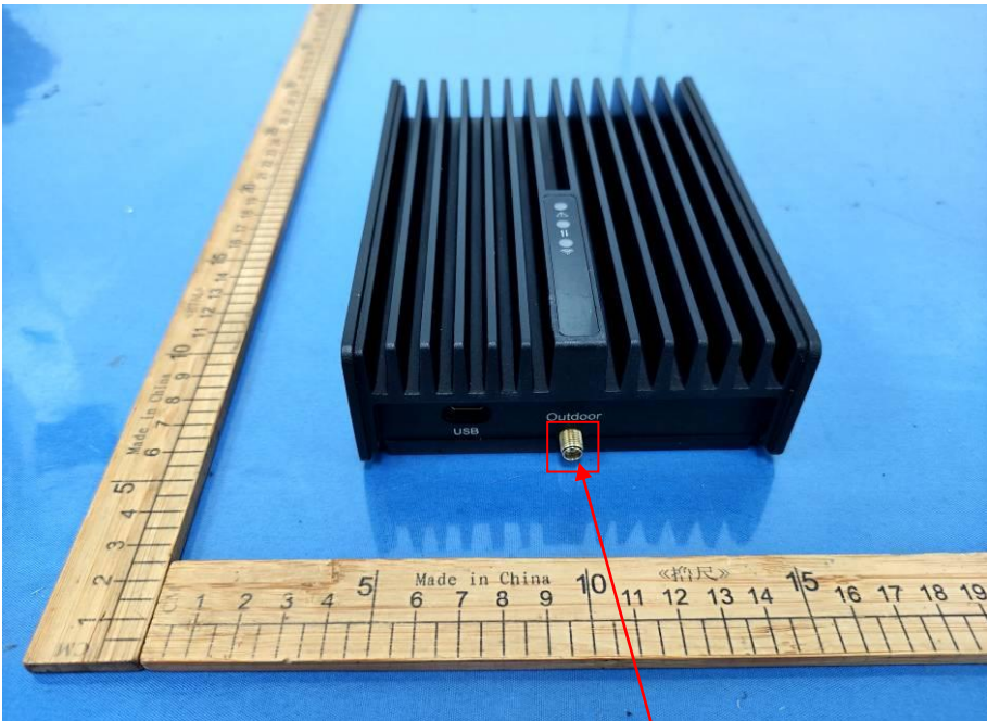
Outdoor Antenna Port
