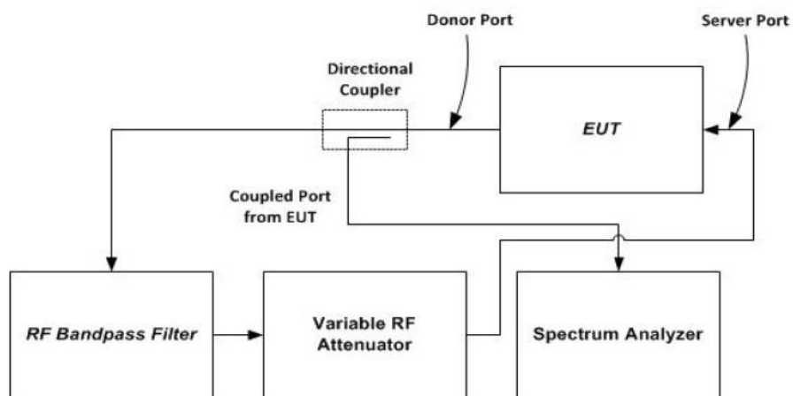
Figure 7 – Oscillation detection instrumentation test setup
