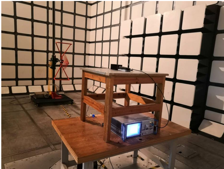
Radiated Emissions View View (Below 1 GHz)
