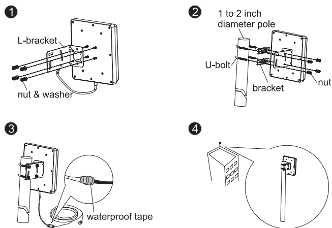
Outdoor wide band panel antenna installation for reference
