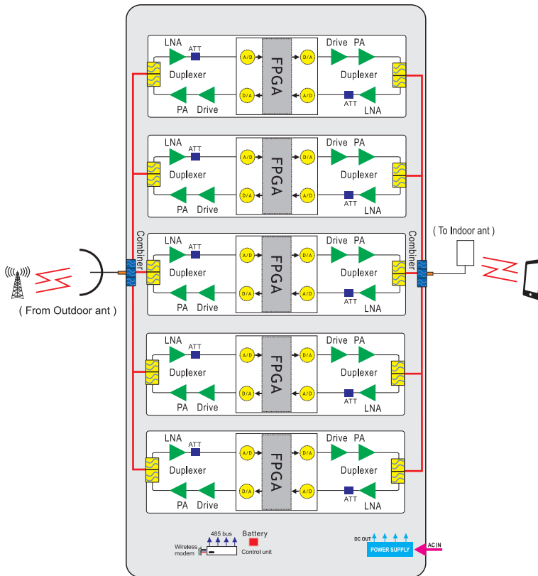
Quint Band block diagram (with remote monitoring)
