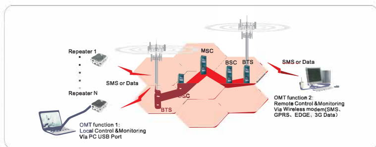
Figure 2: Monitoring function diagram
