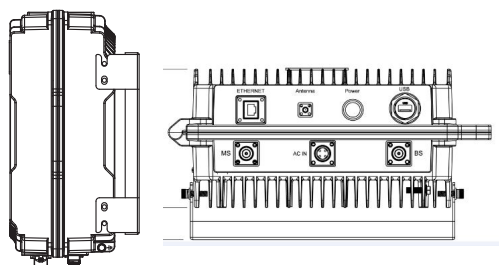
Figure 4: Exterior layout view
