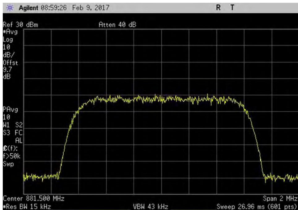
7.10_OBW_DL_869-894MHz_CDMA_Out
