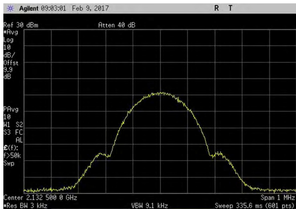
7.10_OBW_DL_2110-2155MHz_GSM_Out
