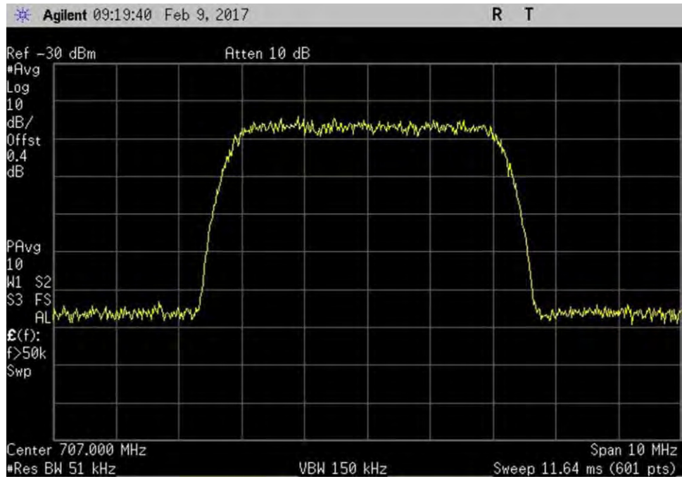
7.10_OBW_UL_698-716MHz_WCDMA_In
