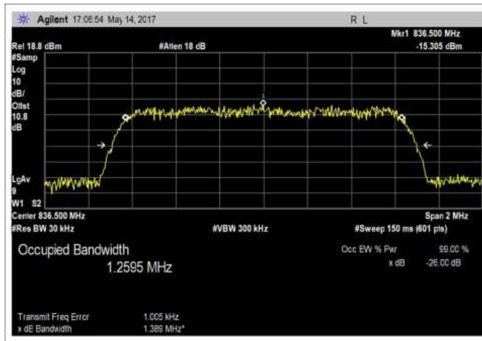
Output_OBW_UL_824-849MHz_CDMA
