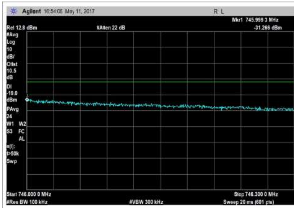
DL_728-746MHz_H_PreAGC_CDMA
