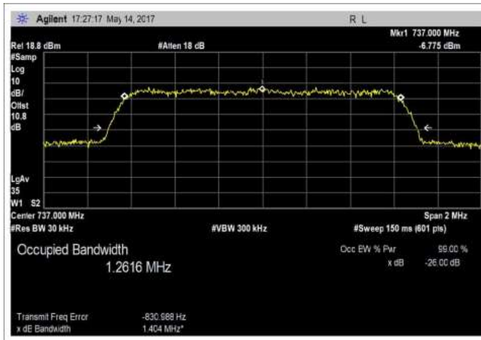
Output_OBW_DL_728-746MHz_CDMA
