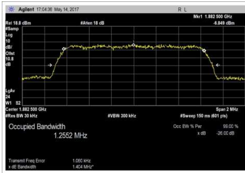
Output_OBW_UL_1850-1915MHz_CDMA
