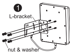
Outdoor wide band directional antenna installation for reference
