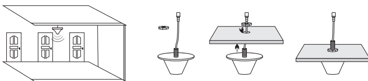
Indoor wide band dome antenna installation for reference
