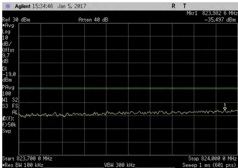
7.5_OBE_UL_824-849MHz_L_PreAGC_CDMA
