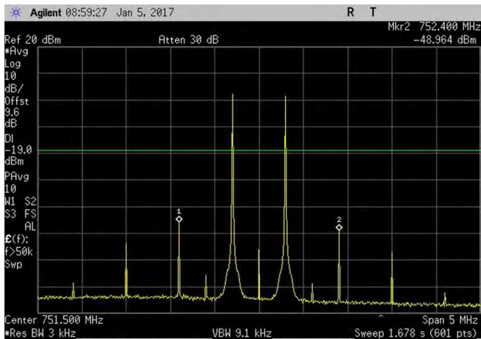
7.4_Intermod_DL_746-757MHz
