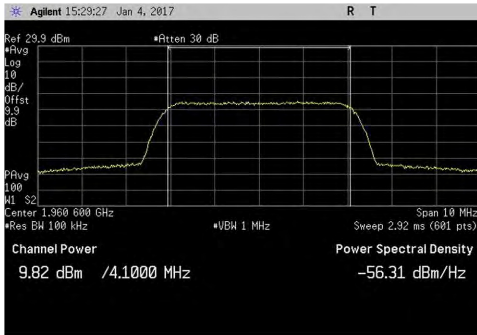
7.2_Power_DL_1930-1995MHz_AWGN
