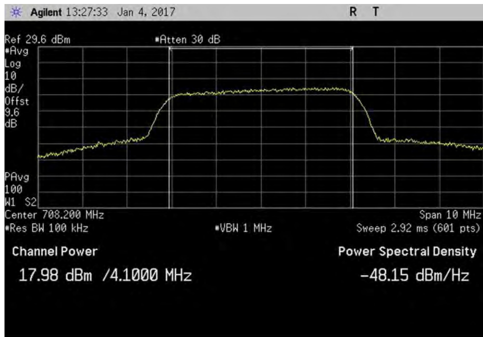
7.2_Power_UL_698-716MHz_AWGN
