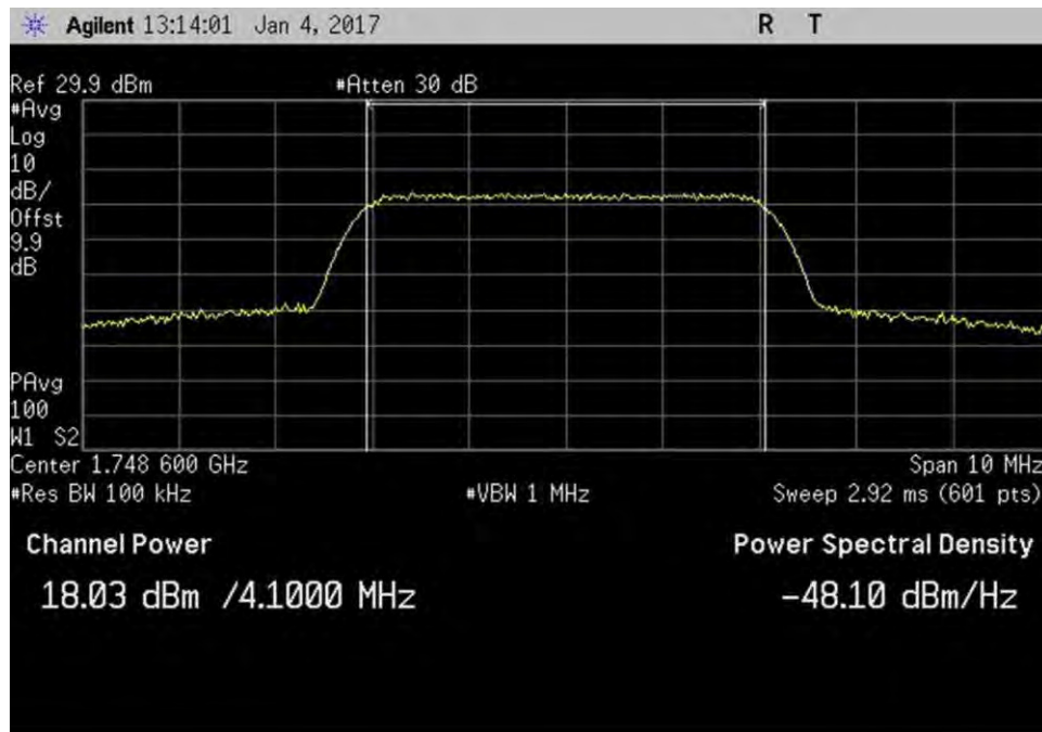
7.2_Power_UL_1710-1755MHz_AWGN
