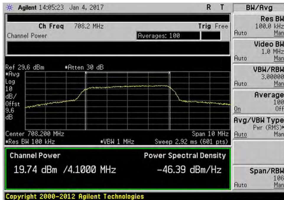
7.2_Power_UL_698-716MHz_AWGN_Max
