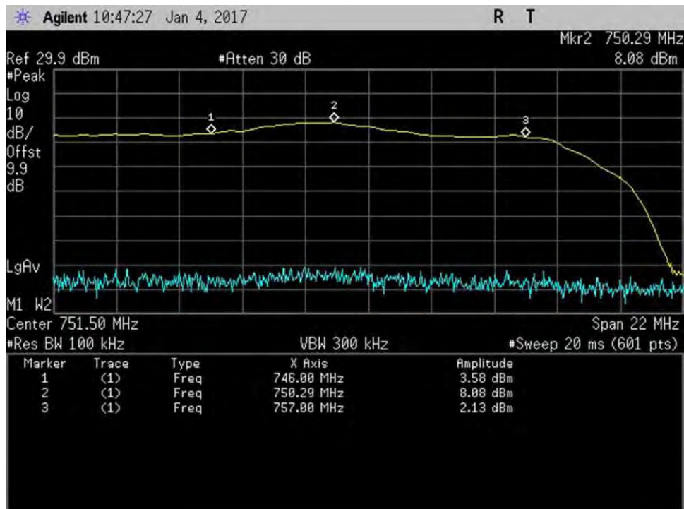
7.1_Band Verify_DL_746-757MHz
