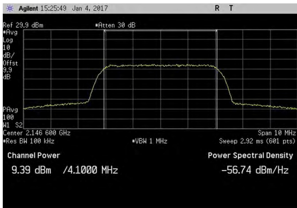
7.2_Power_DL_2110-2155MHz_AWGN_Max
