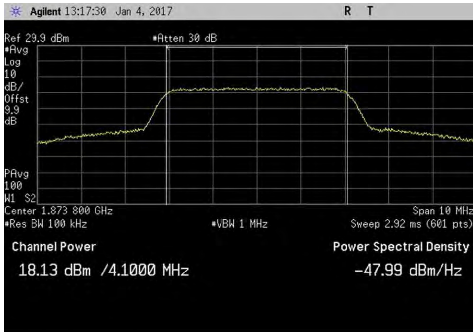
7.2_Power_UL_1850-1915MHz_AWGN
