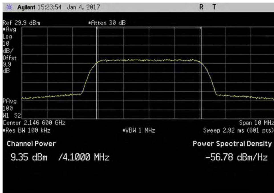
7.2_Power_DL_2110-2155MHz_AWGN
