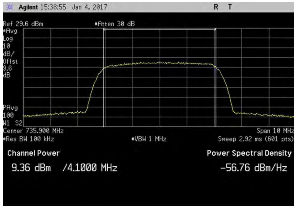
7.2_Power_DL_728-746MHz_AWGN
