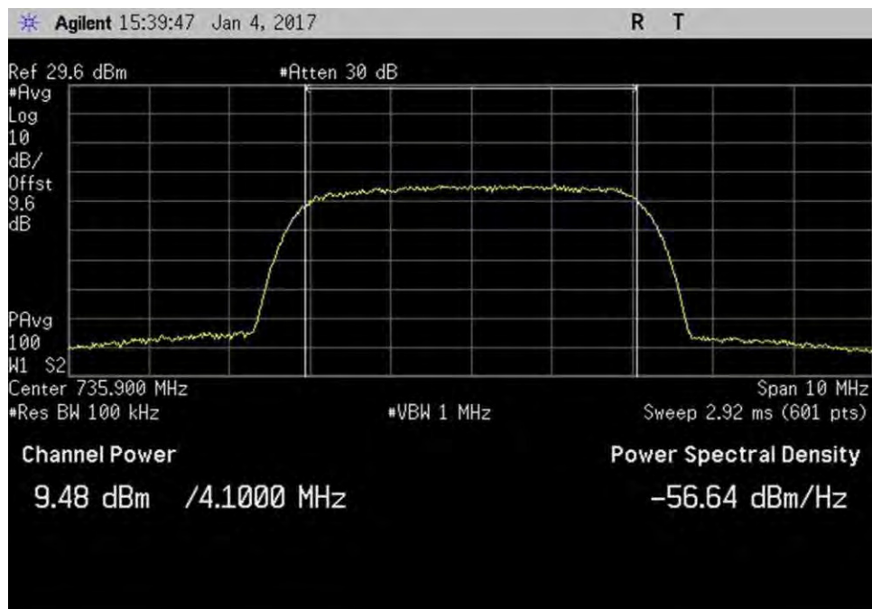
7.2_Power_DL_728-746MHz_AWGN_Max
