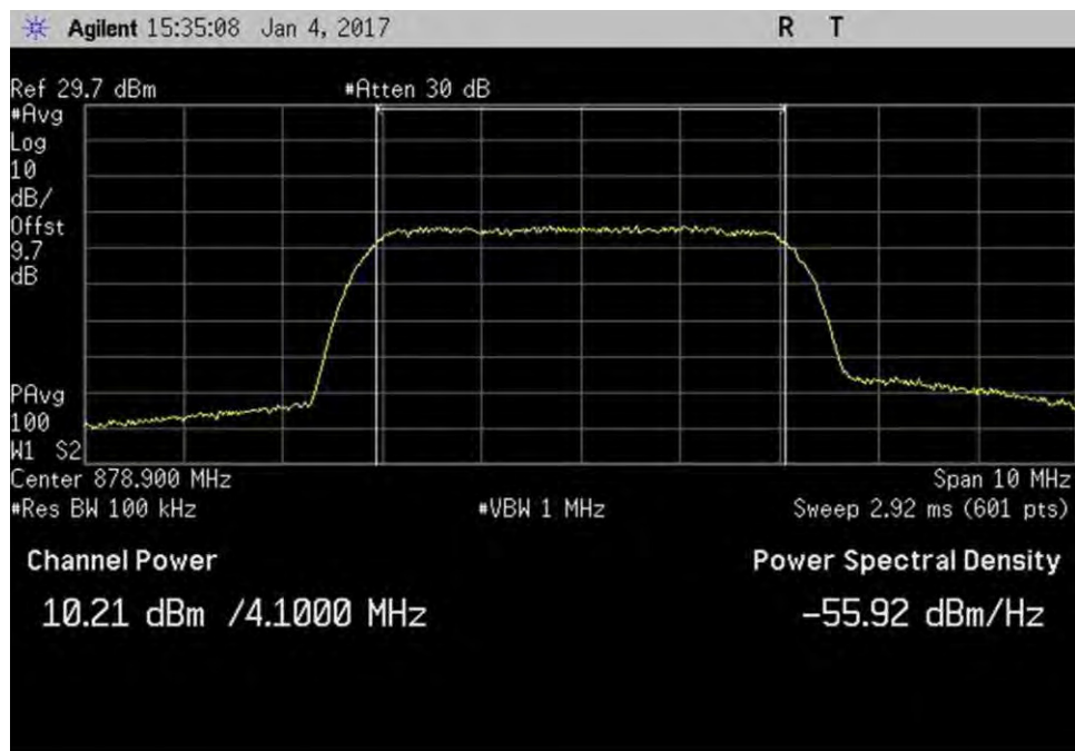
7.2_Power_DL_869-894MHz_AWGN_Max
