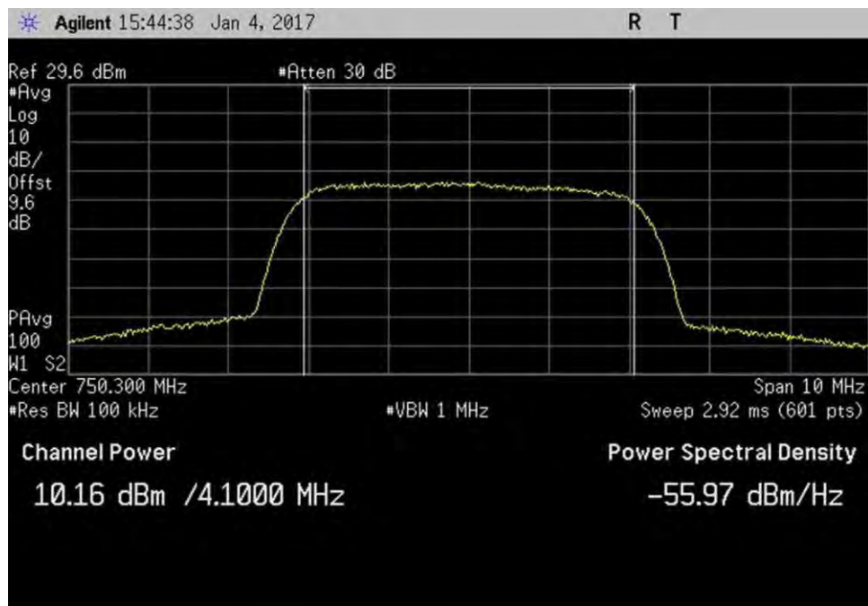
7.2_Power_DL_746-757MHz_AWGN_Max
