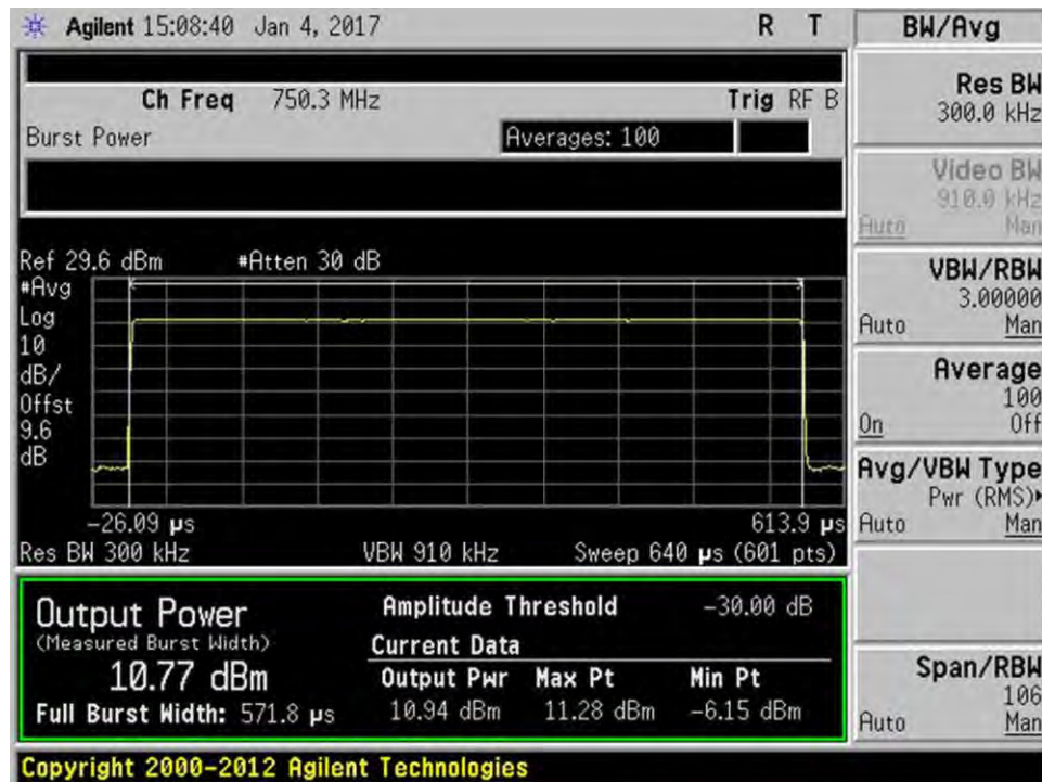
7.2_Power_DL_746-757MHz_GSM
