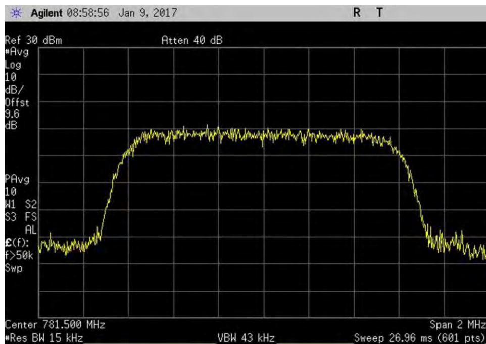
7.10_OBW_UL_776-787MHz_CDMA_Out
