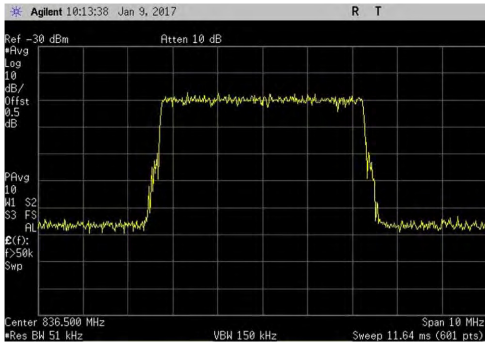
7.10_OBW_UL_824-849MHz_LTE_In
