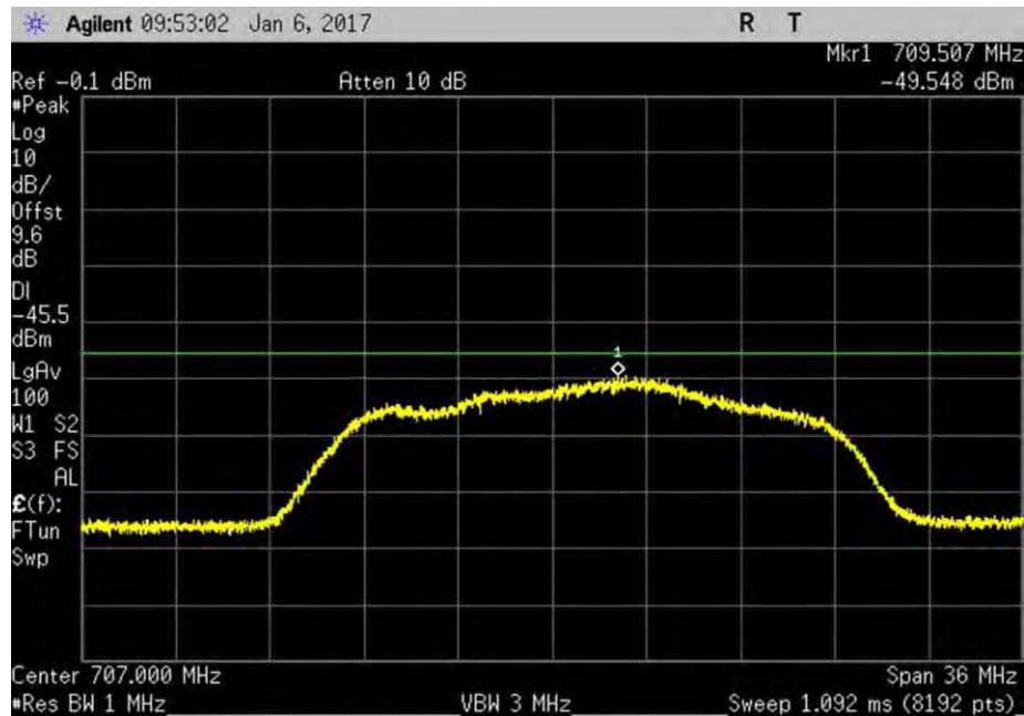
7.7.1_Noise_UL_698-716MHz
