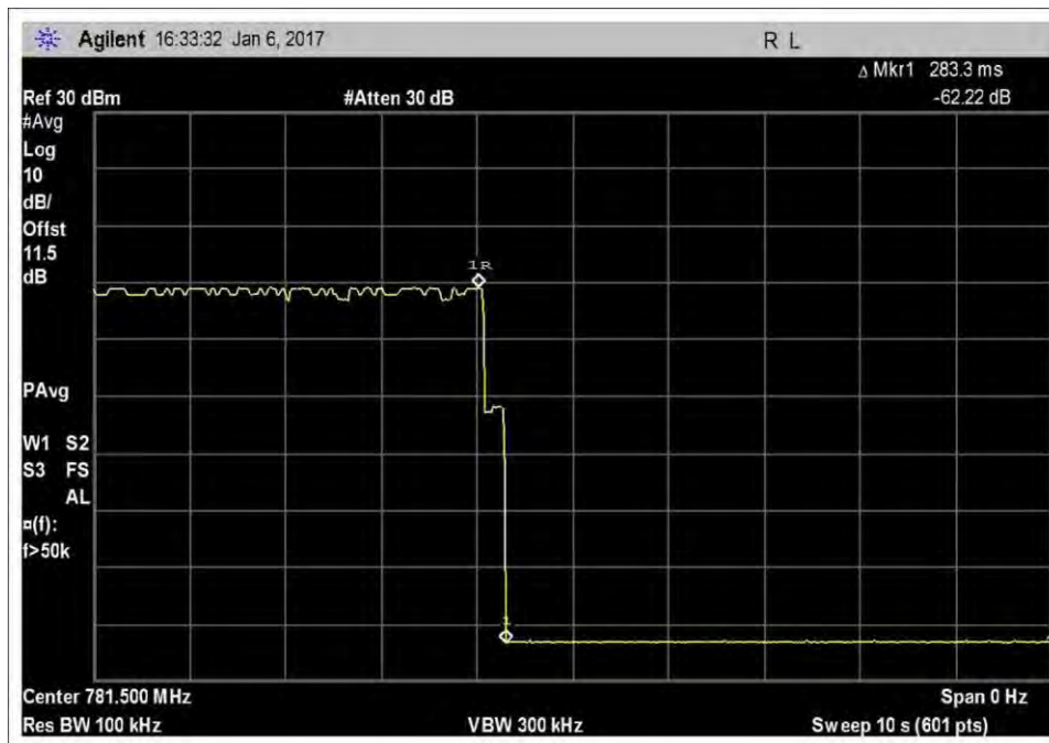
7.9.2_VarULGainTiming_UL_776-787MHz
