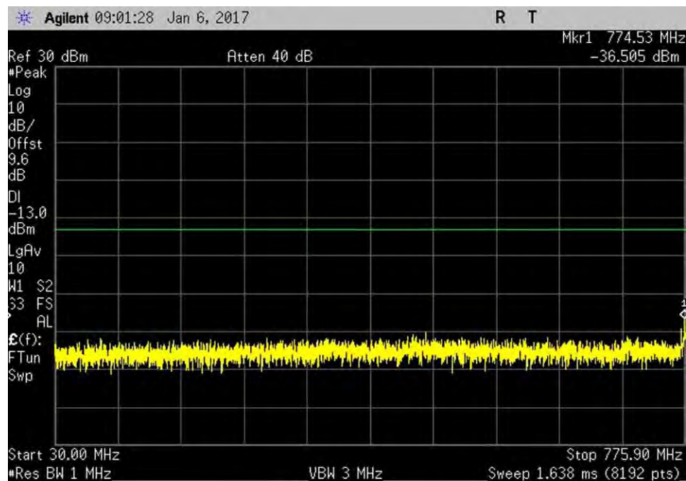
7.6_CSE_UL_776-787MHz_L
