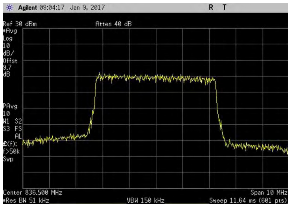
7.10_OBW_UL_824-849MHz_LTE_Out
