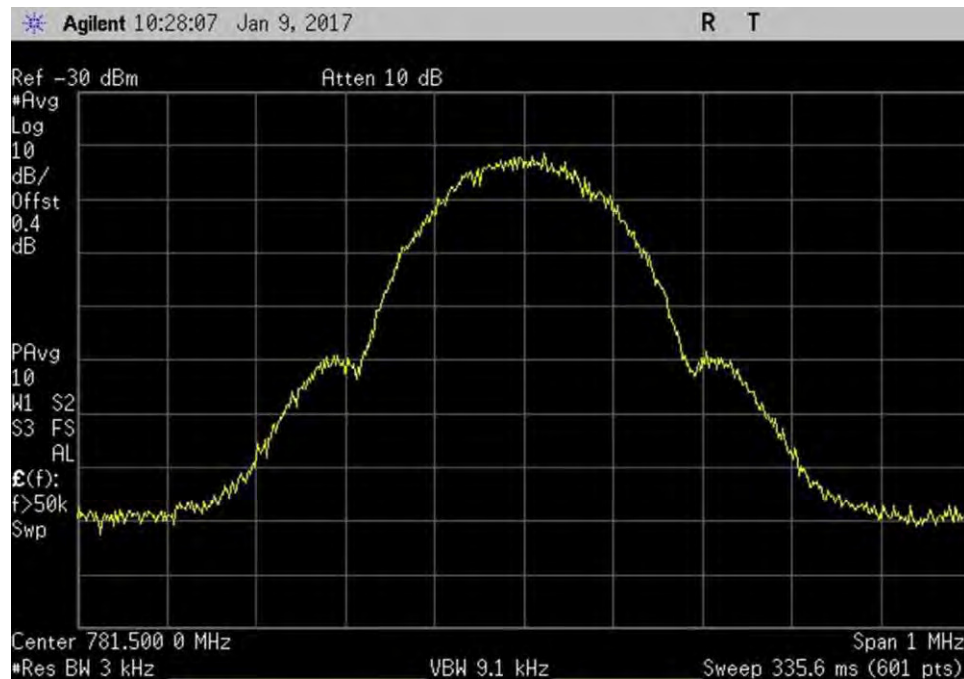
7.10_OBW_UL_776-787MHz_GSM_In
