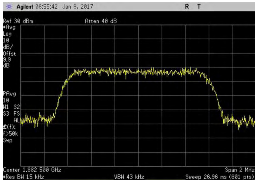
7.10_OBW_UL_1850-1915MHz_CDMA_Out
