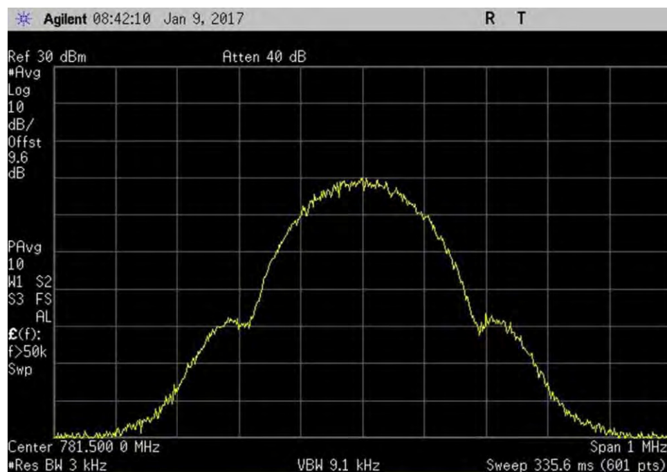
7.10_OBW_UL_776-787MHz_GSM_Out
