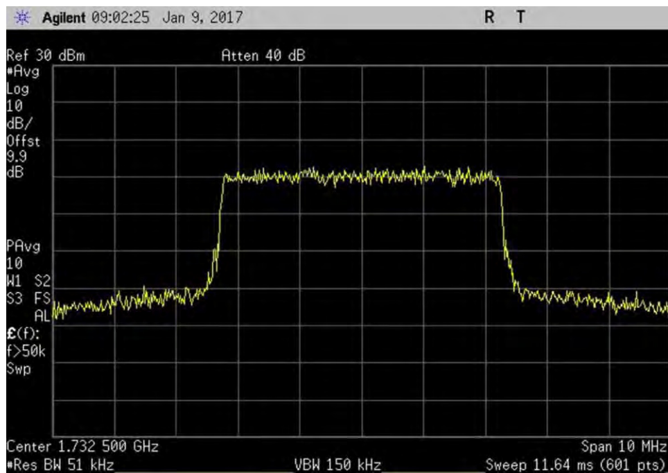
7.10_OBW_UL_1710-1755MHz_LTE_Out
