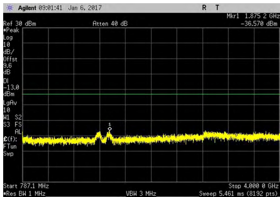
7.6_CSE_UL_776-787MHz_R1
