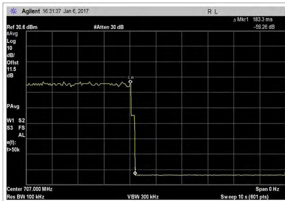
7.9.2_VarULGainTiming_UL_698-716MHz
