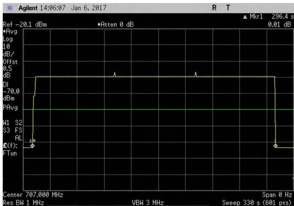
7.8_Inactivity_UL_698-716MHz
