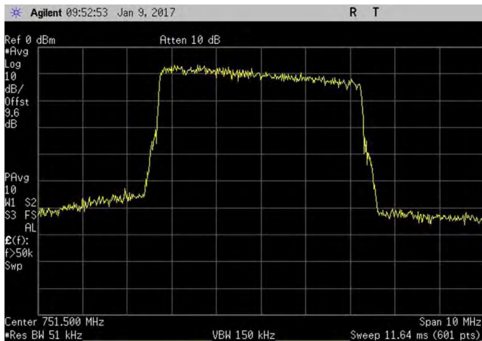
7.10_OBW_DL_746-757MHz_LTE_Out
