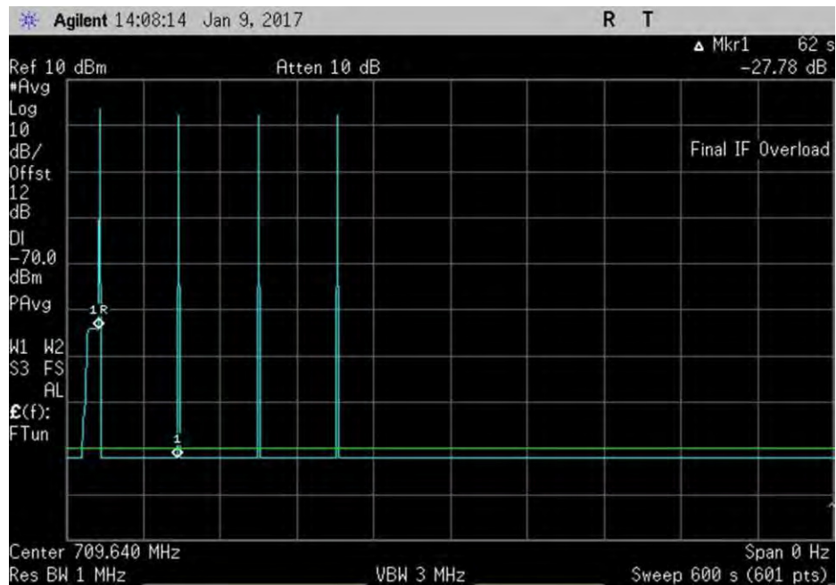
7.11.2_osc_UL_698-716MHz600sec
