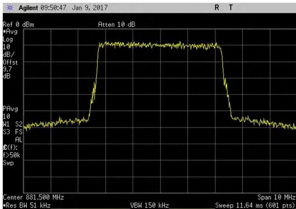
7.10_OBW_DL_869-894MHz_LTE_Out
