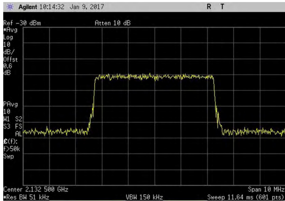
7.10_OBW_DL_2110-2155MHz_LTE_In
