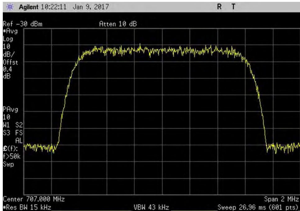
7.10_OBW_UL_698-716MHz_CDMA_In
