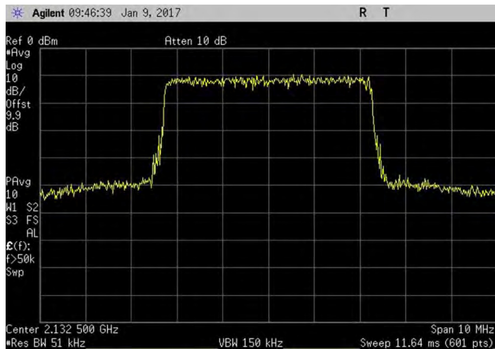
7.10_OBW_DL_2110-2155MHz_LTE_Out
