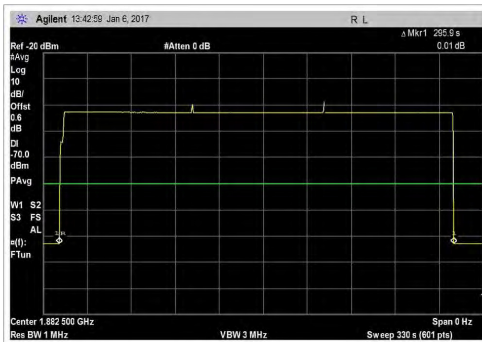
7.8_Inactivity_UL_1850-1915MHz
