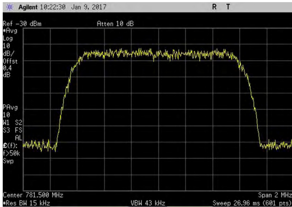
7.10_OBW_UL_776-787MHz_CDMA_In
