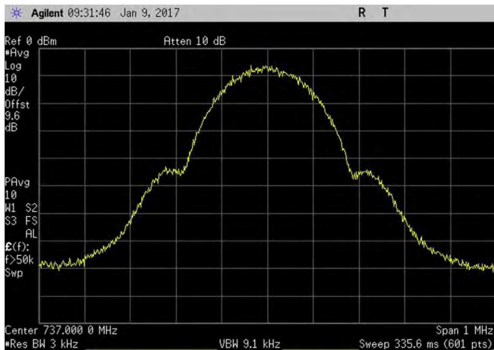
7.10_OBW_DL_728-746MHz_GSM_Out
