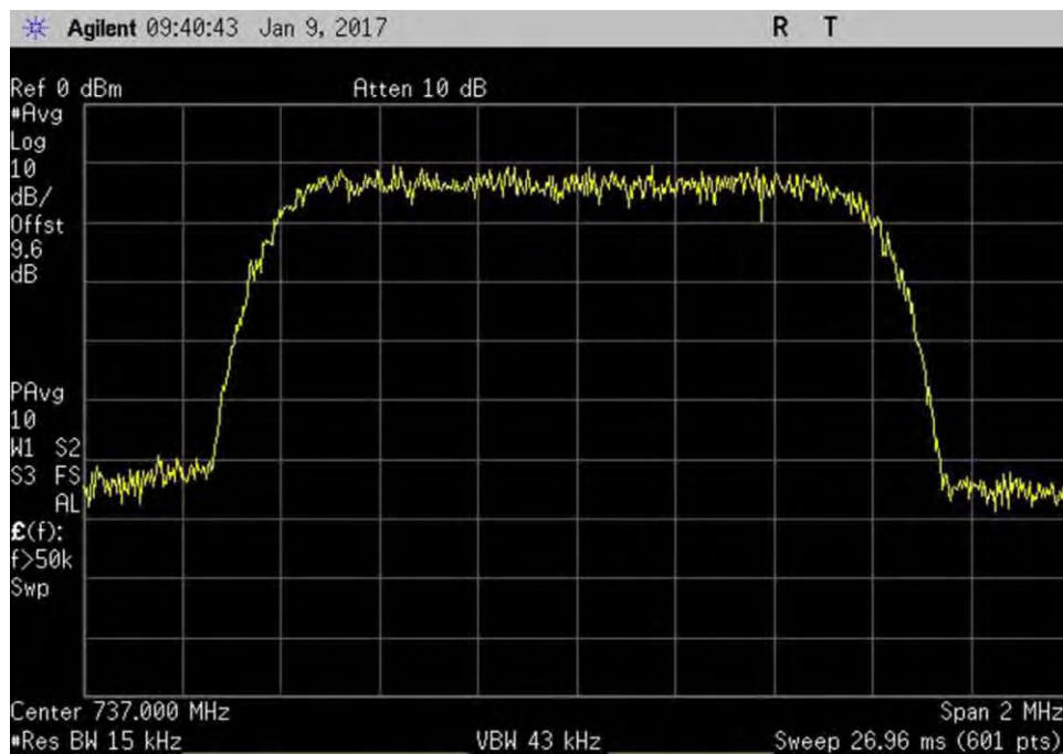
7.10_OBW_DL_728-746MHz_CDMA_Out
