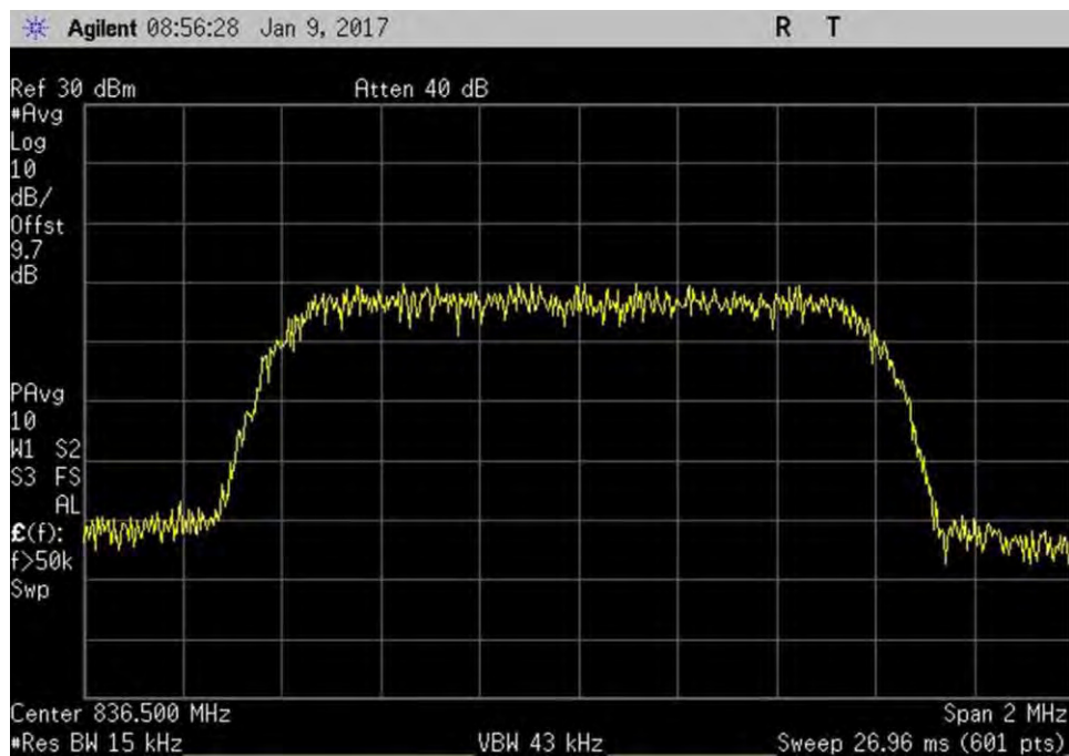
7.10_OBW_UL_824-849MHz_CDMA_Out
