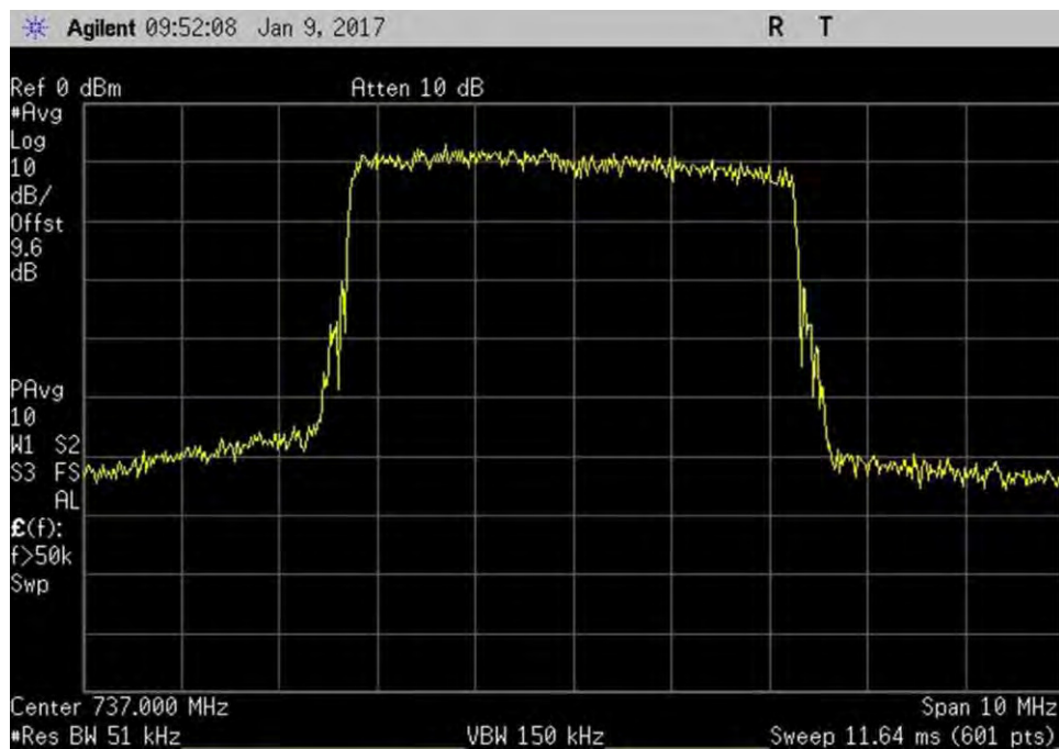
7.10_OBW_DL_728-746MHz_LTE_Out
