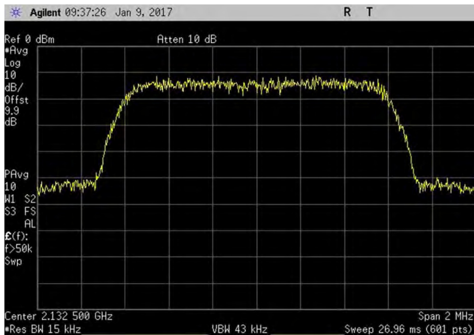
7.10_OBW_DL_2110-2155MHz_CDMA_Out
