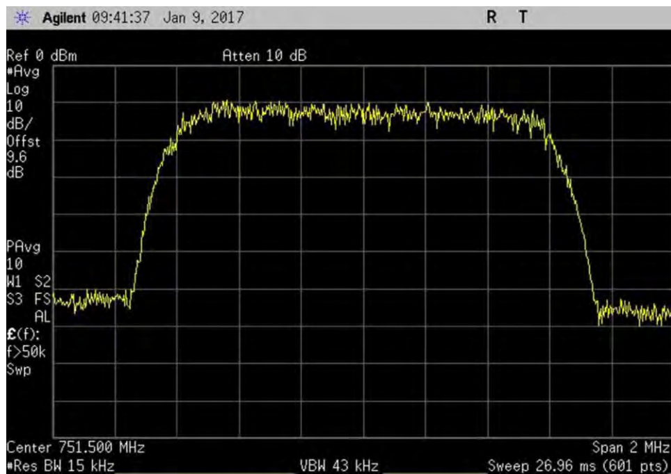
7.10_OBW_DL_746-757MHz_CDMA_Out
