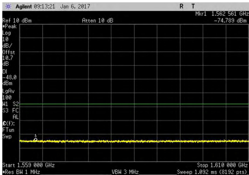
7.6_CSE_UL_776-787MHz_GPSwFilter
