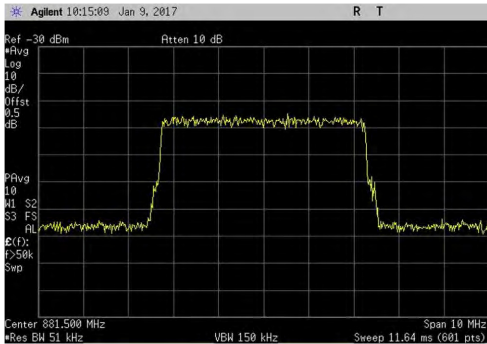
7.10_OBW_DL_869-894MHz_LTE_In
