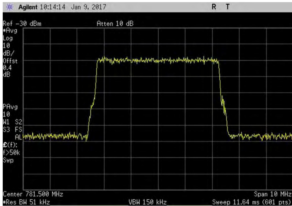
7.10_OBW_UL_776-787MHz_LTE_In
