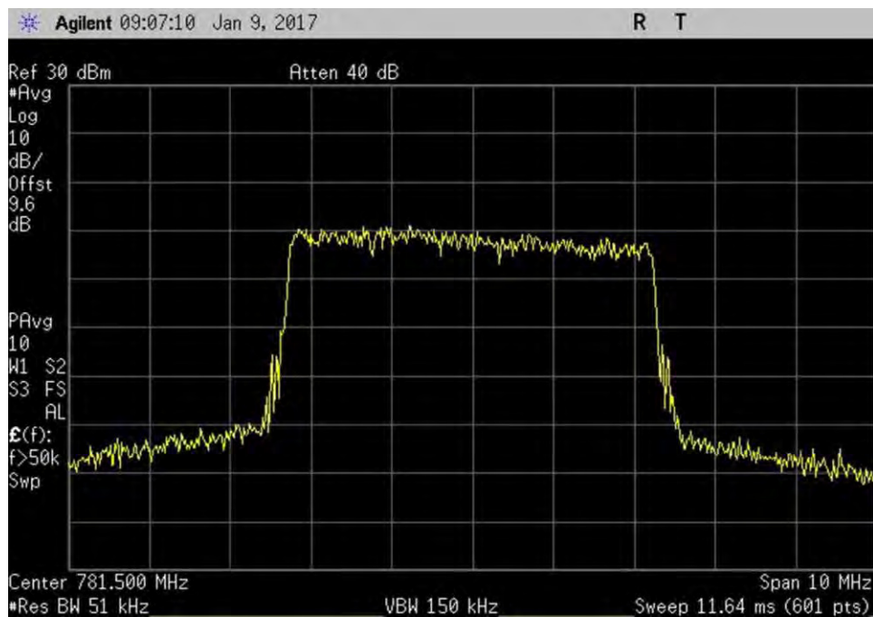
7.10_OBW_UL_776-787MHz_LTE_Out
