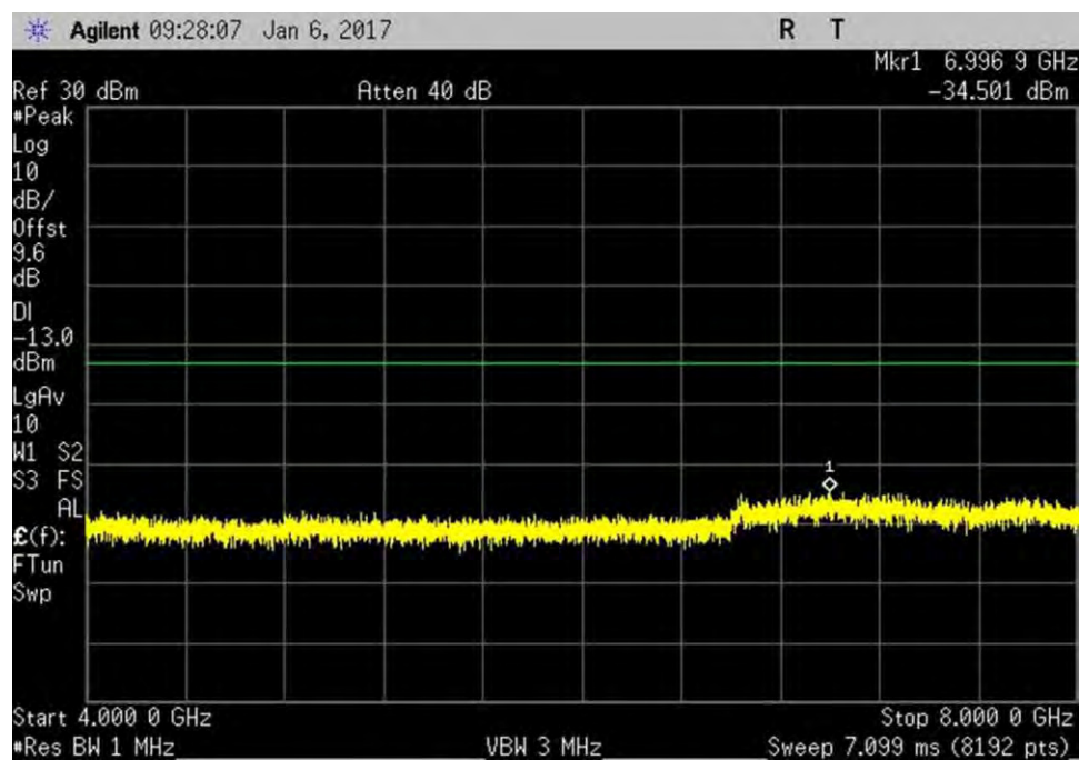
7.6_CSE_DL_746-757MHz_R2
