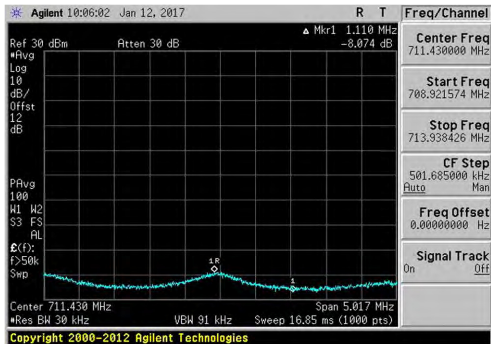
7.11.3_Osc_UL_698-716MHz+5_AWGNL
