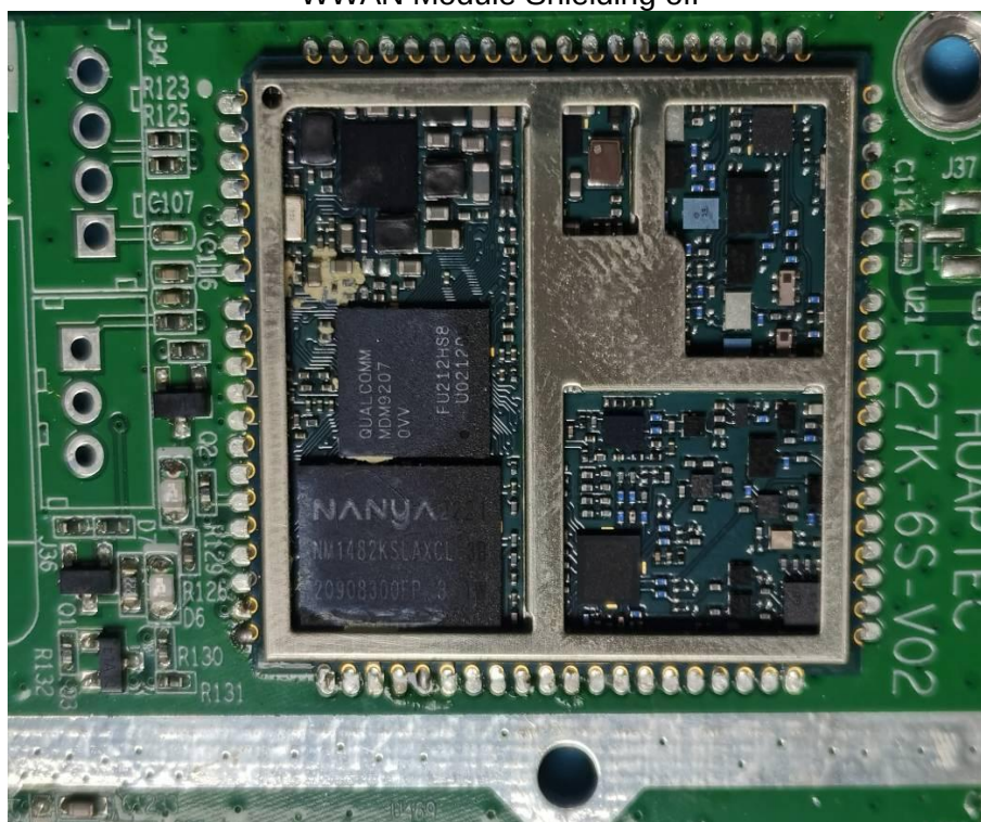
WWAN Module Shielding off
