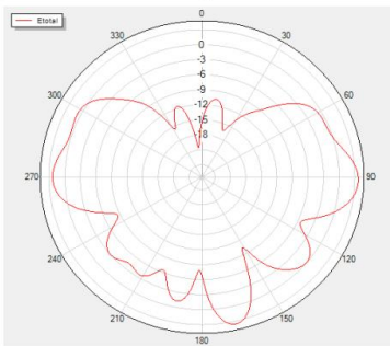
Phi=90 Freq=5150MHz
