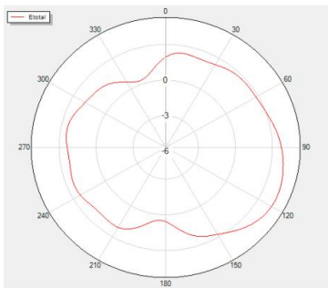
Theta=90 Freq=5150MHz
