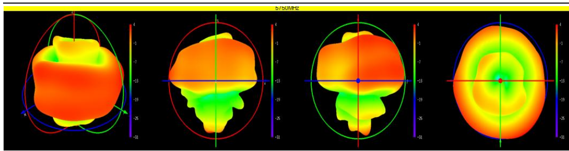
Theta=90 Freq=5750MHz
