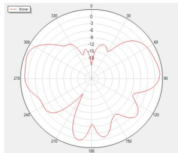
Phi=0 Freq=5350MHz
