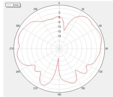
Phi=0 Freq=2500MHz
