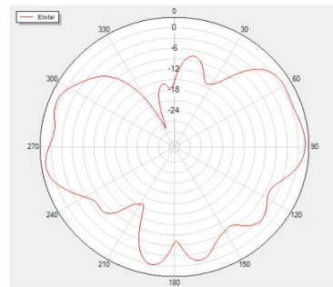
Phi=0 Freq=5150MHz
