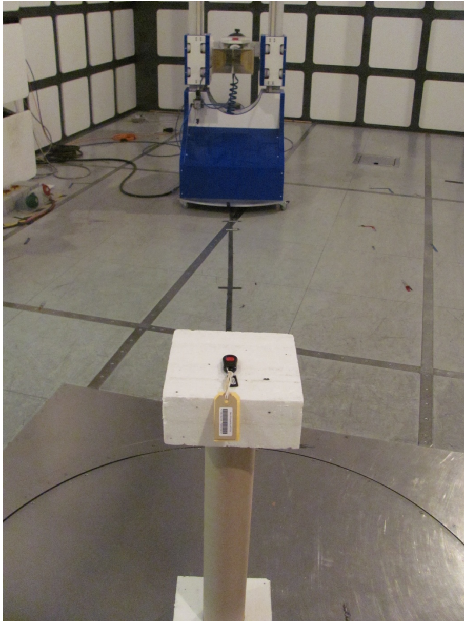
Radiated Emissions 1-5GHz
