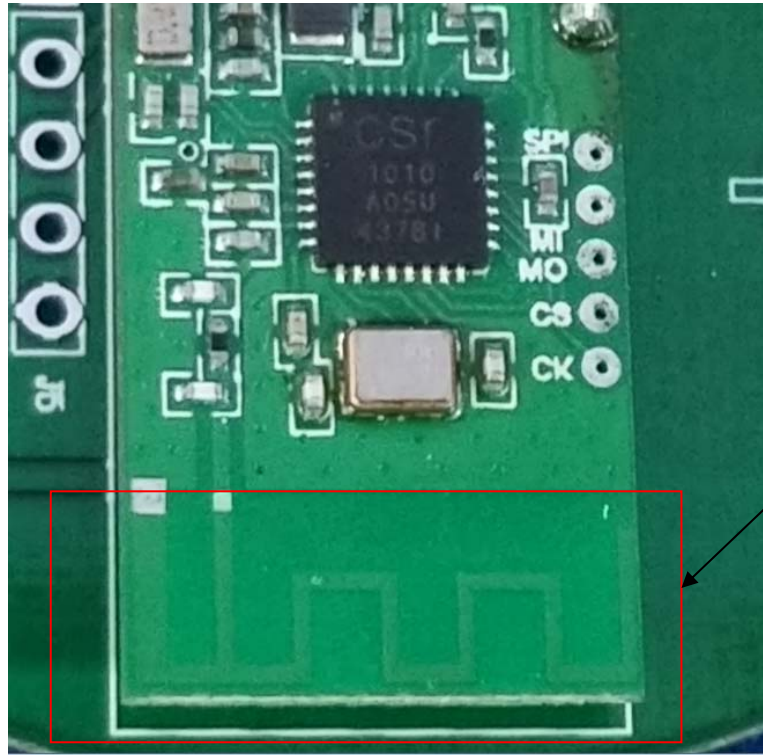
Bluetooth Antenna
