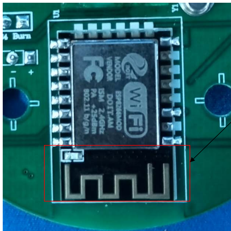
Wi-Fi Antenna
