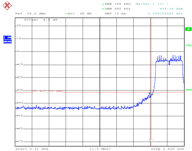
802.11n(HT20) Low Band Edge Plot
