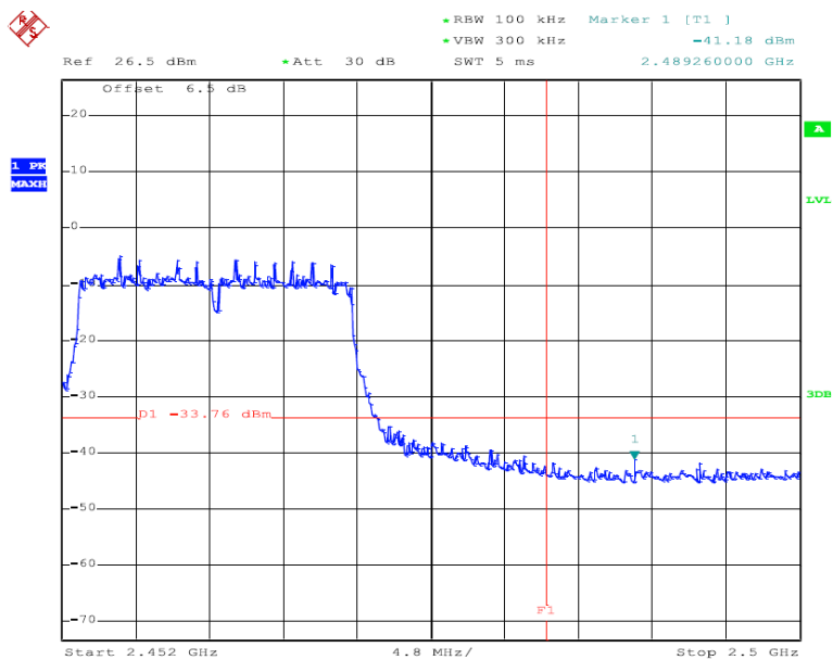
802.11n(HT20) High Band Edge Plot
