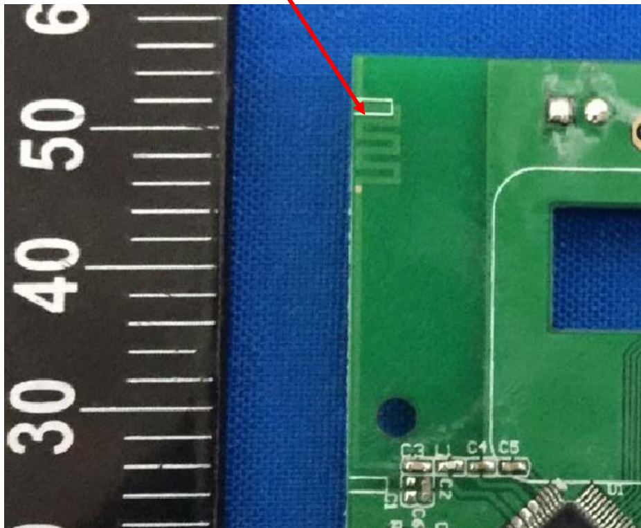
PCB Antenna – View
