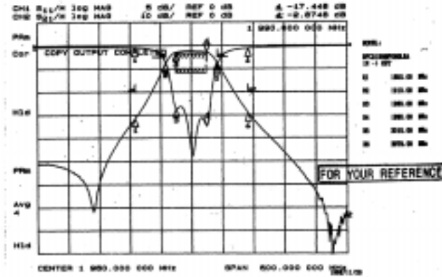
(1) Typical Frequency Response of Bass Filter #1 (FL2001)
