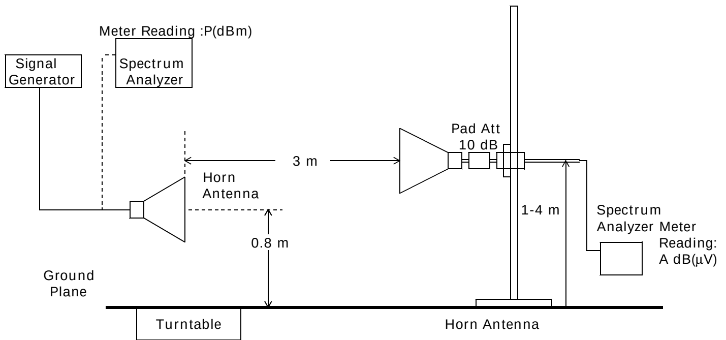
(c-2) Substitution Horn Antenna
