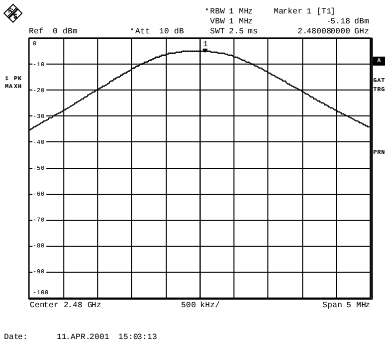
Plot 2 – Peak power on highest channel with 3.3V and at +25°C.
