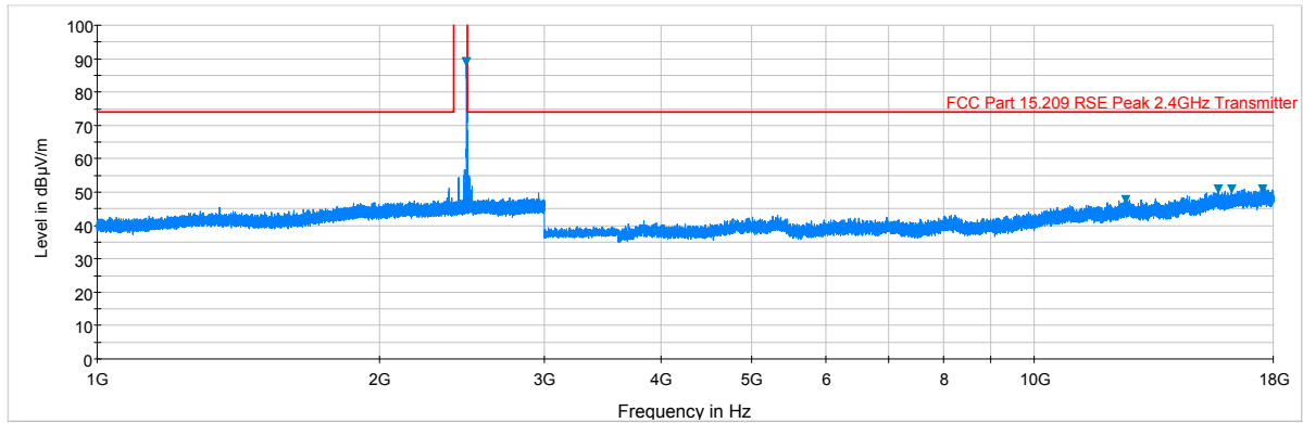
Plot 6-7. Radiated Spurious Plot above 1GHz (BTLE – Ch. 19, Ant. Pol. V)
