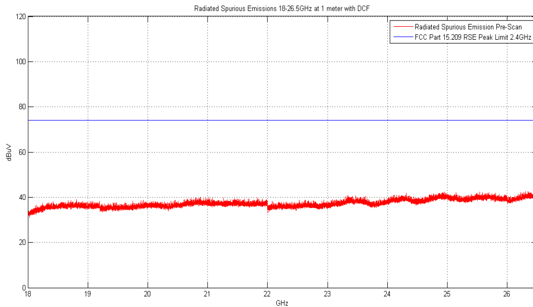
Plot 6-11. Radiated Spurious Plot above 18GHz (Pol. V)
