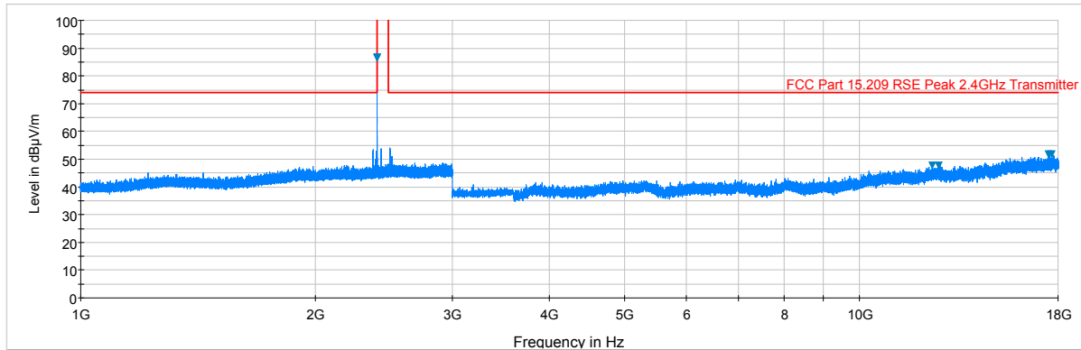
Plot 6-4. Radiated Spurious Plot above 1GHz (BTLE – Ch. 0, Ant. Pol. H)
