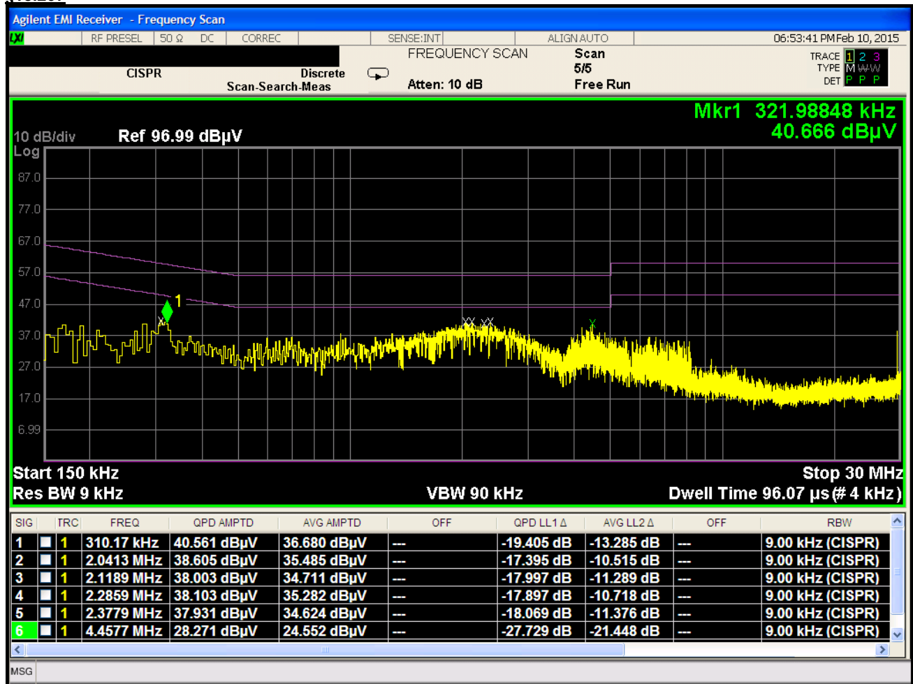
Plot 6-14. Line-Conducted Test Plot (L1)
