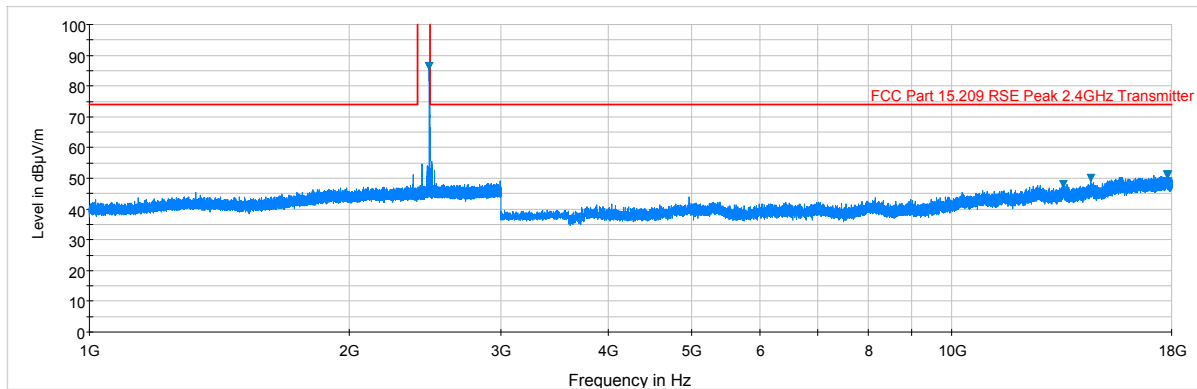
Plot 6-6. Radiated Spurious Plot above 1GHz (BTLE – Ch. 19, Ant. Pol. H)
