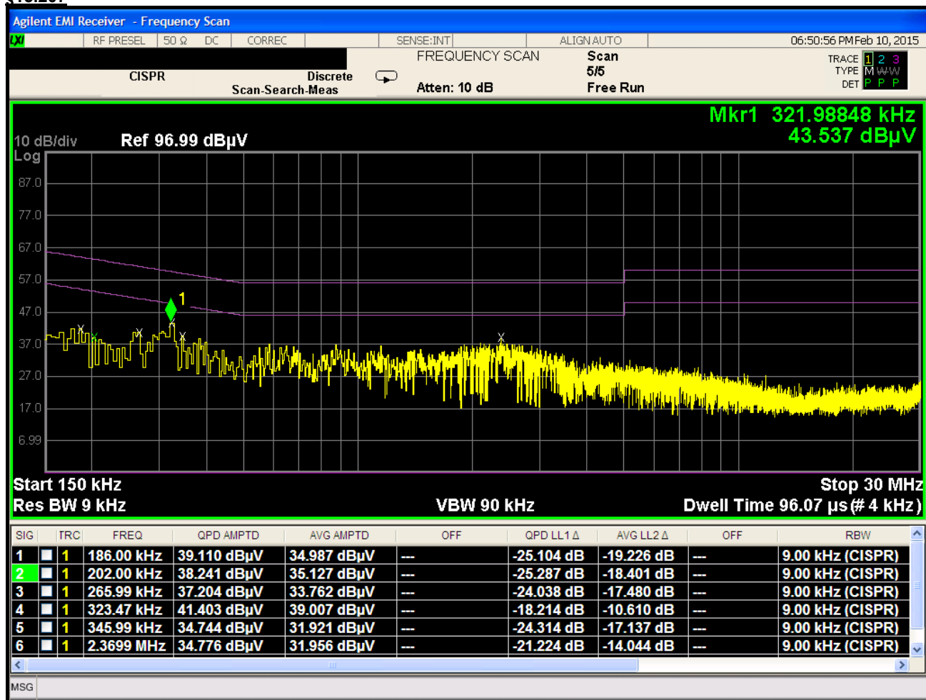
Plot 6-15. Line-Conducted Test Plot (N)
