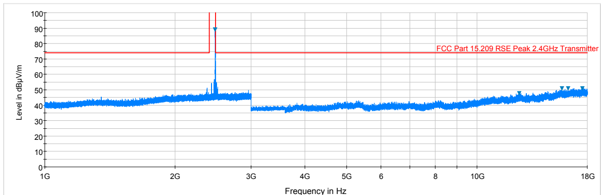
Plot 6-9. Radiated Spurious Plot above 1GHz (BTLE – Ch. 39, Ant. Pol. V)
