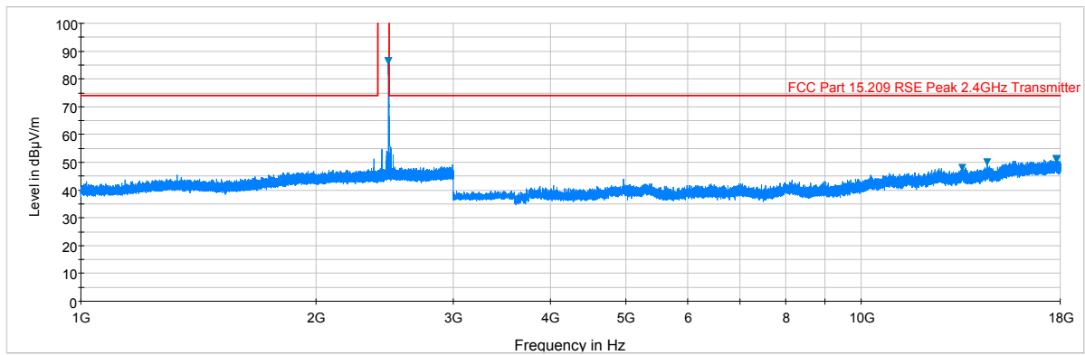
Plot 6-8. Radiated Spurious Plot above 1GHz (BTLE – Ch. 39, Ant. Pol. H)
