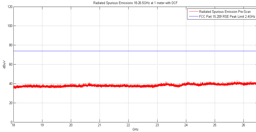
Plot 6-10. Radiated Spurious Plot above 18GHz (Pol. H)
