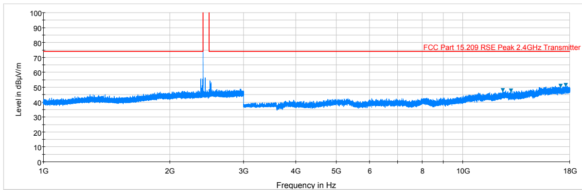
Plot 6-5. Radiated Spurious Plot above 1GHz (BTLE – Ch. 0, Ant. Pol. V)
