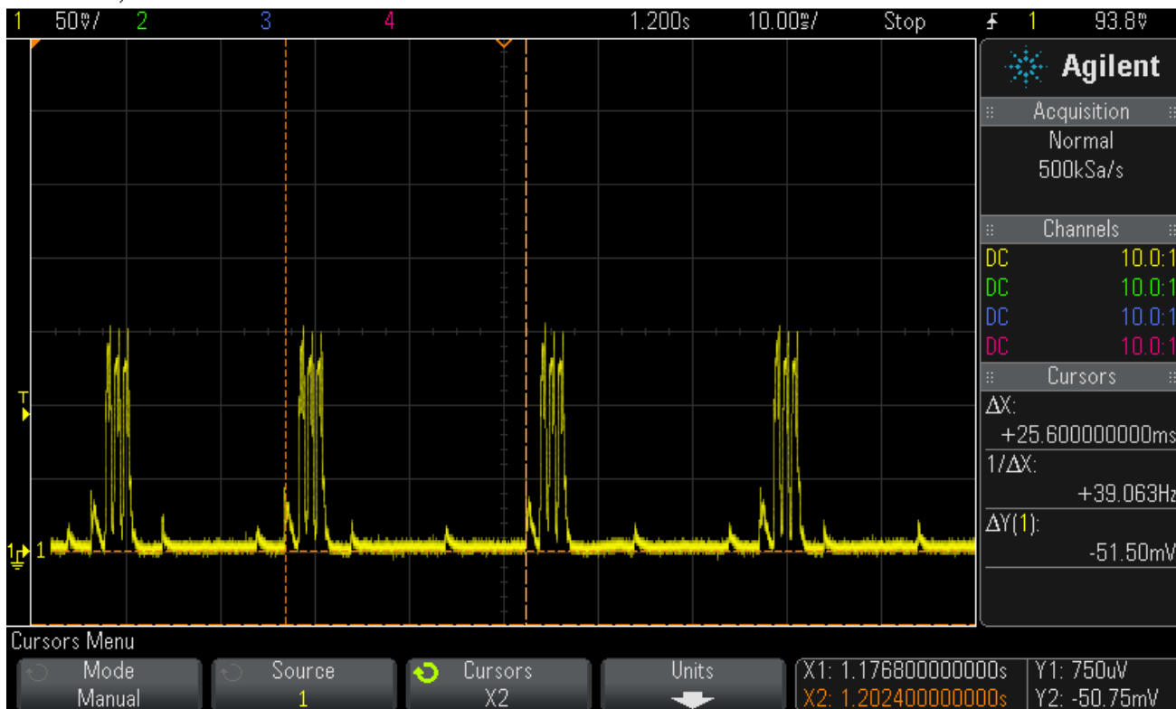
Plot 6-3. Worst Case 100ms Operation
