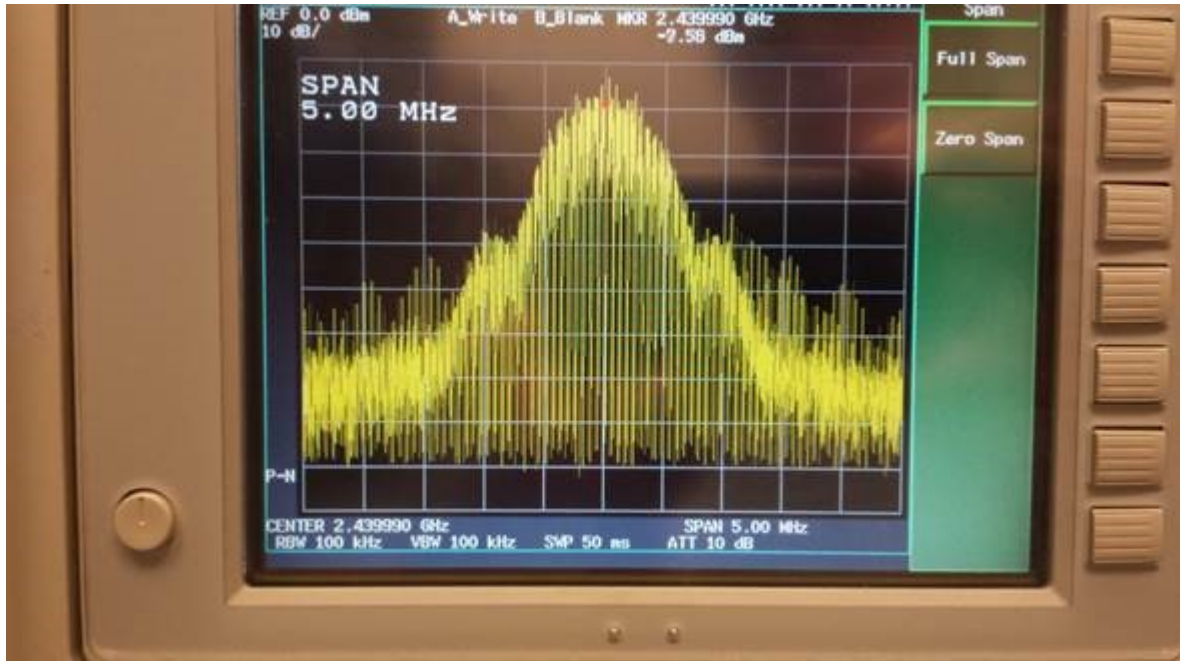
Figure 8-1. Occupied Bandwidth Plot (BTLE – Ch. 19)
