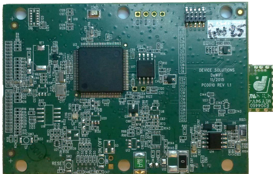
WiFi Radio Board – Top:
