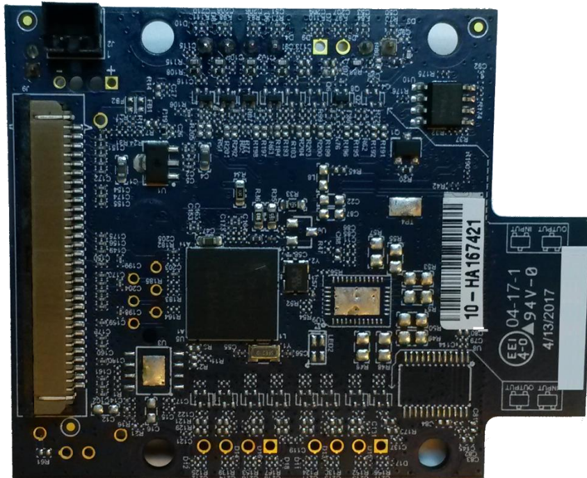
ISM Radio Board – Bottom:
