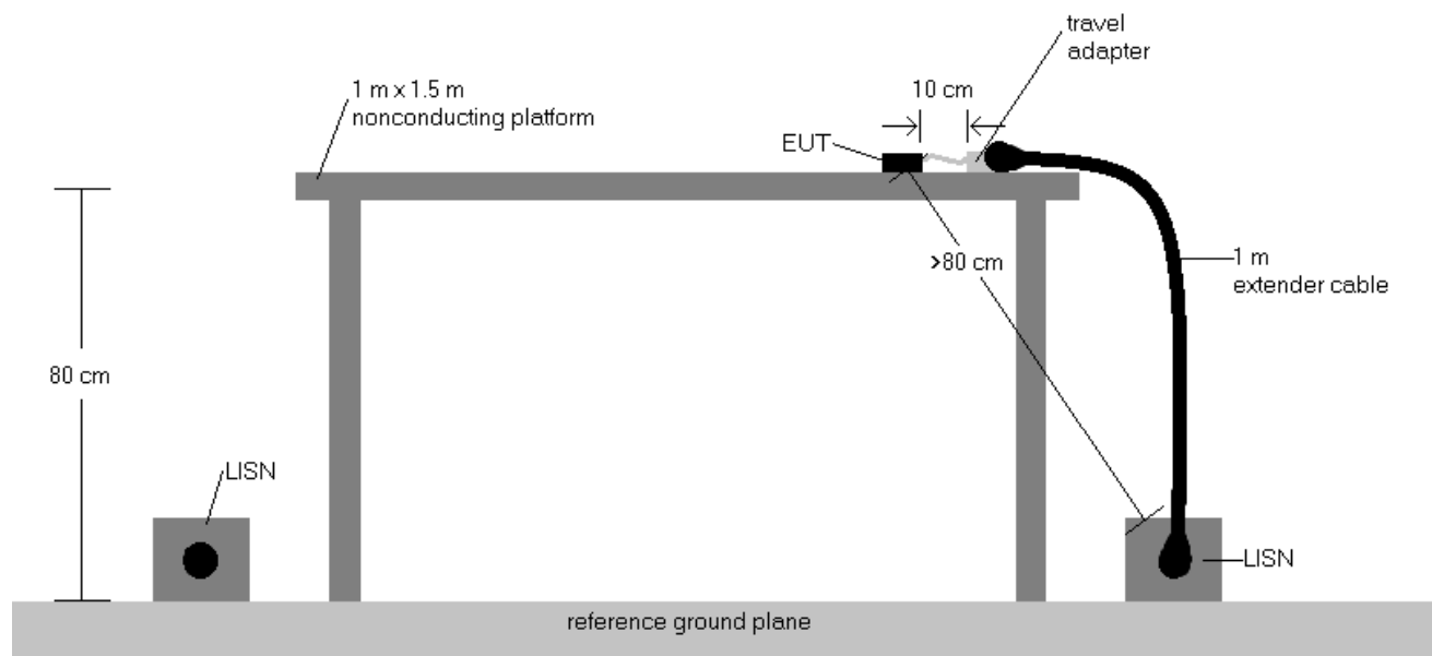
Figure 7-4. Test Instrument & Measurement Setup
