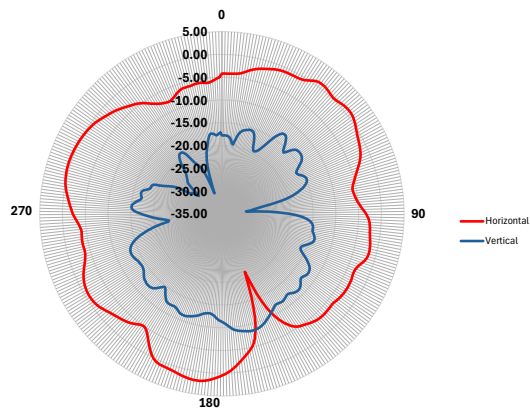
ANTENNA 1 - YX Cut Antenna Gain (dBi)
