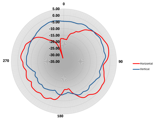
ANTENNA 1 - YZ Cut Antenna Gain (dBi)
