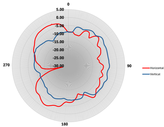
ANTENNA 2 - ZX Cut Antenna Gain (dBi)
