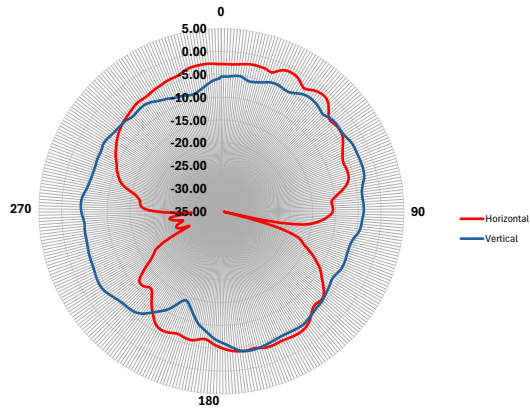
ANTENNA 1 - ZX Cut Antenna Gain (dBi)
