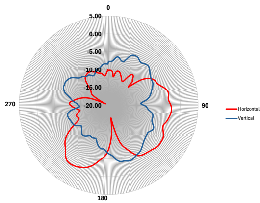
ANTENNA 2 - YZ Cut Antenna Gain (dBi)
