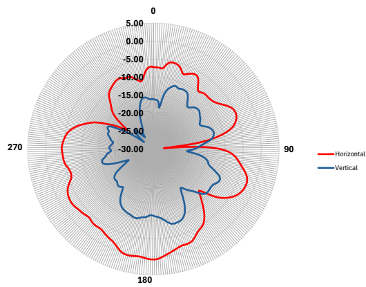
ANTENNA 2 - YX Cut Antenna Gain (dBi)
