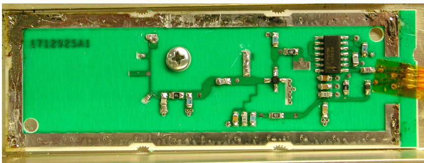
Photo of PV2000 transmitter PCA mounted in antenna housing.
