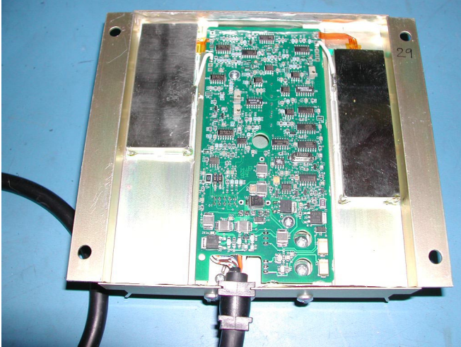
Photo of rear of PV2000 showing signal processing PCA (center) surrounded by shielded transmitter PCA (right side) and receiver PCA (left side).
