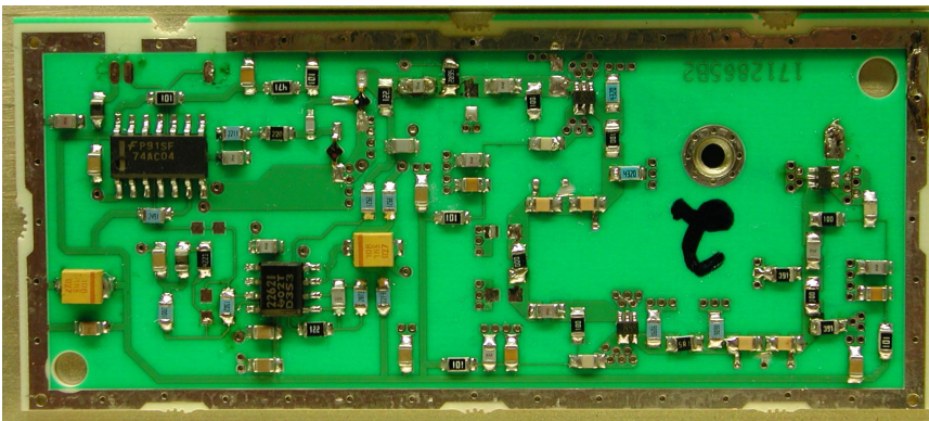
Photo of PV2000 transmitter PCA mounted in antenna housing.
