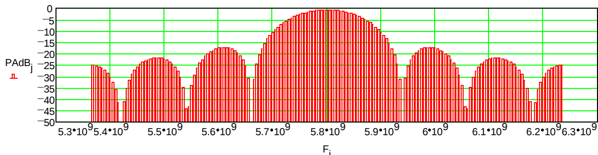
APPROX. MEASURED OUTPUT POWER SPECTRUM Resolution Bandwidth = 130MHz (Full Pulse Spectrum) -> Confirms App-Note 150-2
