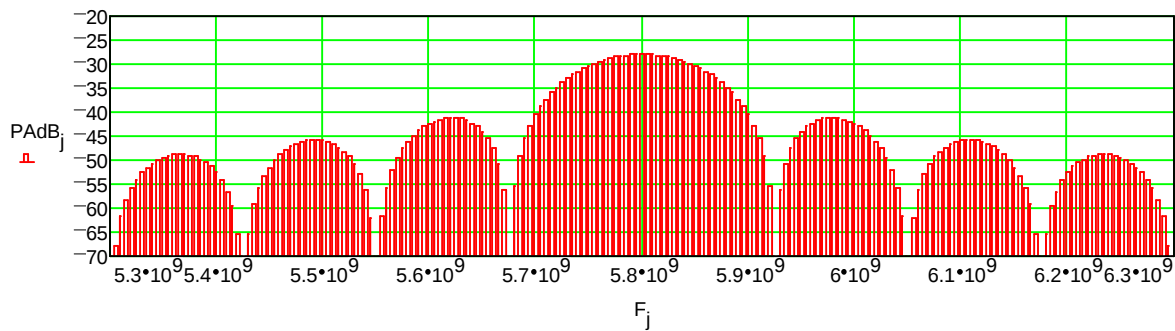
Resolution Bandwidth configured for Full Pulse Spectrum in Accordance with App-Note 150-2 (Note: Must repeat entire equation set for MCAD to recalculate)
