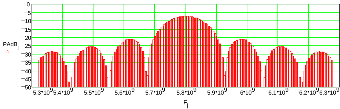
APPROX. MEASURED OUTPUT POWER SPECTRUM Resolution Bandwidth = 50MHz (Realistic Pulse Spectrum)
