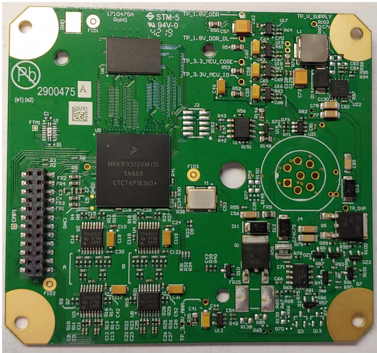
Processor PCA Front
