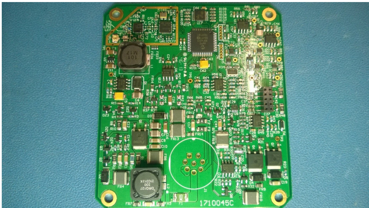
WWS7220 Processor PCB Top
