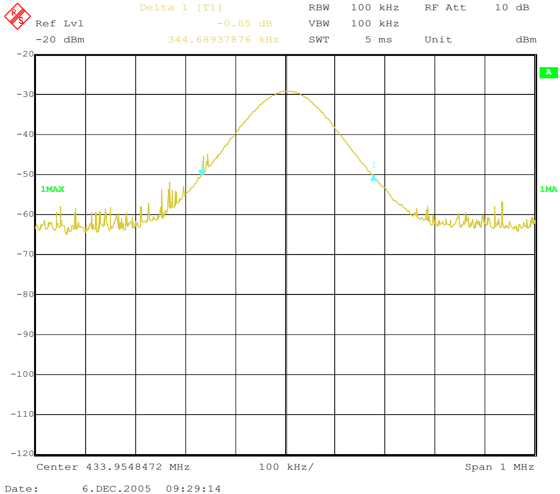
Figure 4-1: Bandwidth plot
