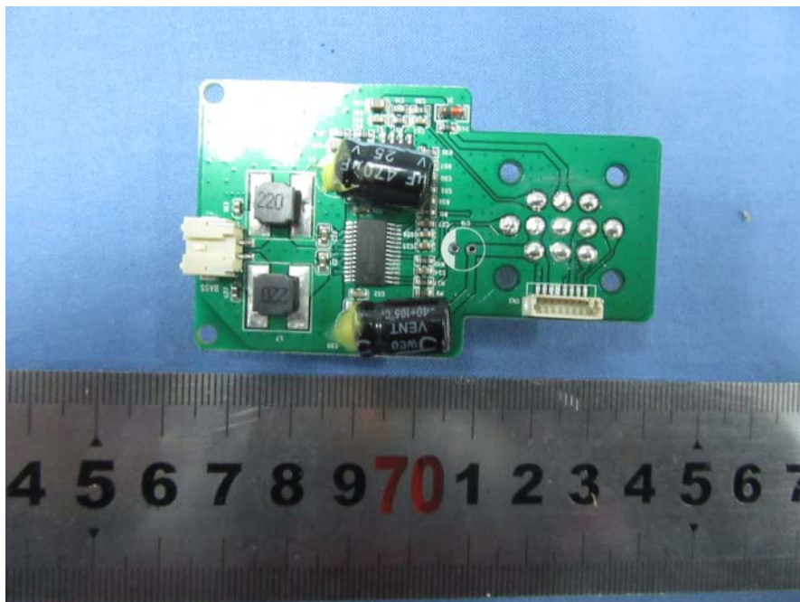
EUT – Base Board Top View
