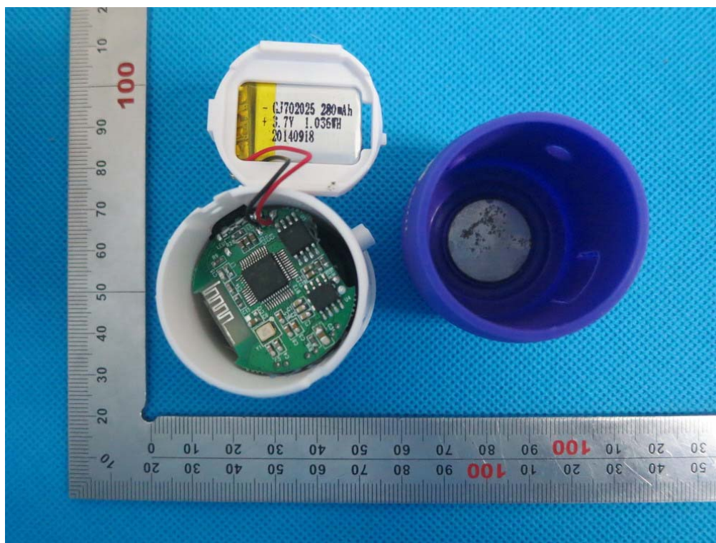
OPEN TOP VIEW OF EUT
