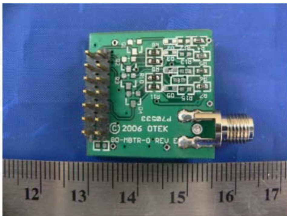
EUT – Board 2 view -2
