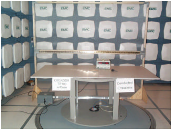
Conducted Emissions Test Set-up
