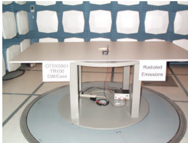
Radiated CW Test Set-up Photos
