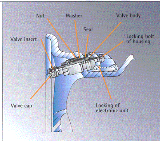
Drawing of the valve with quotation of its special features
