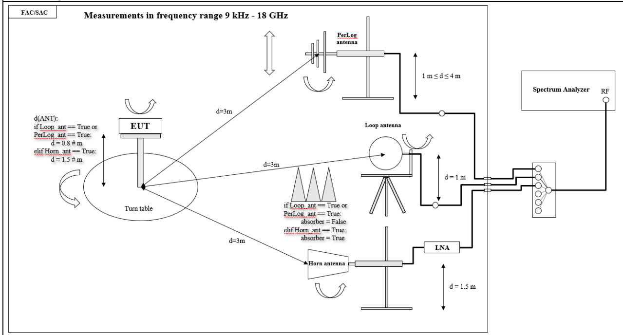
Block diagram 1:
