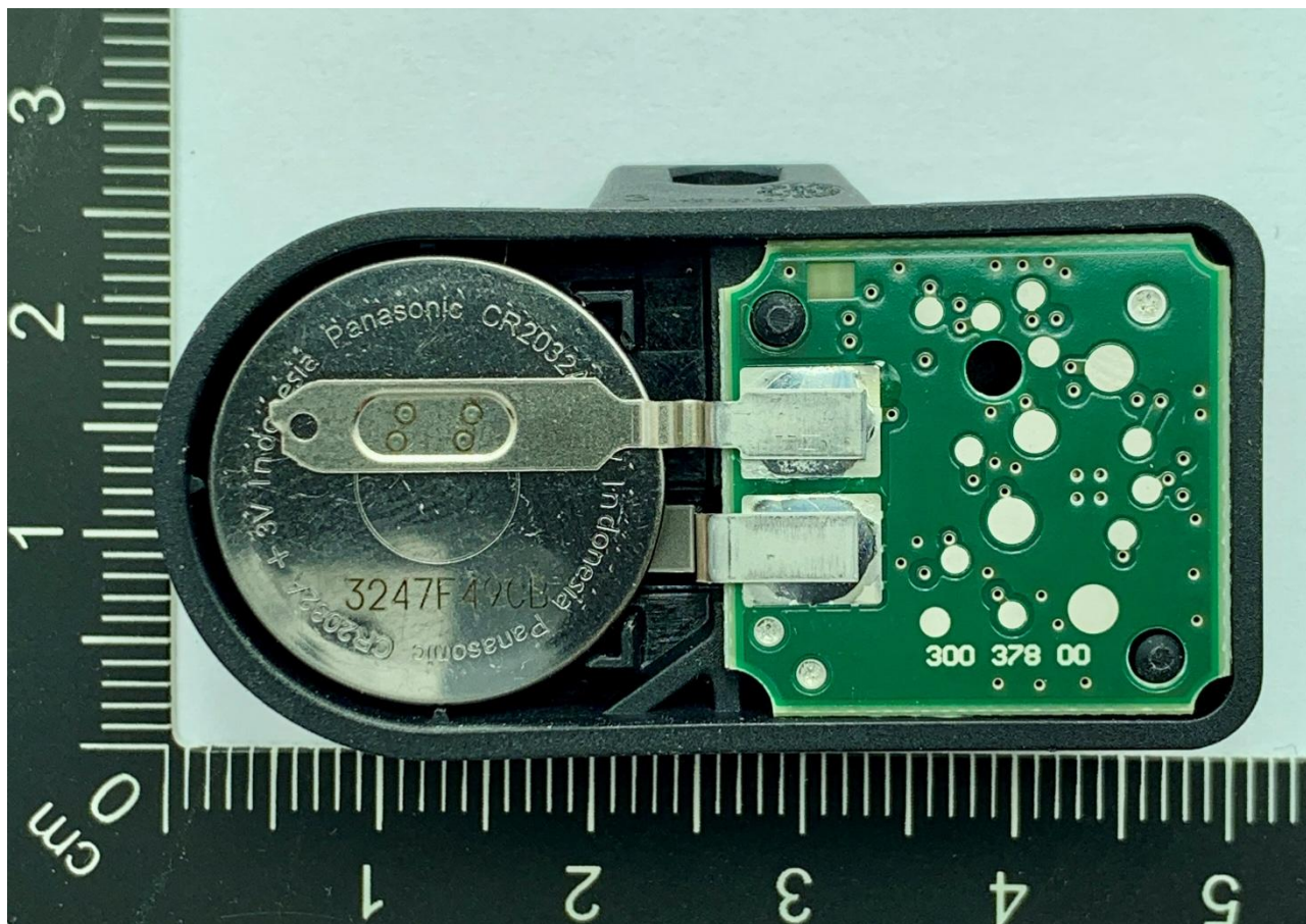
assembly of PCBA, battery and housing
