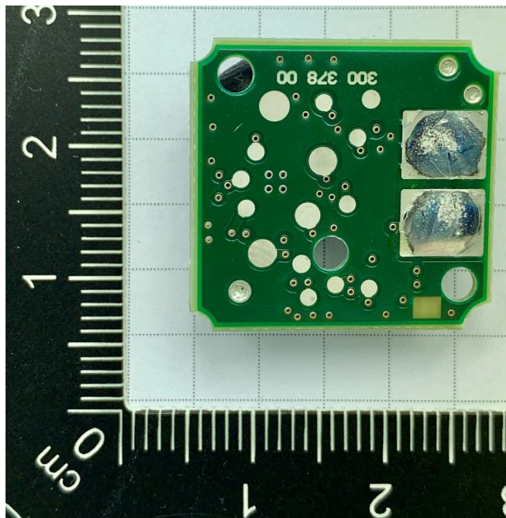
PCB bottom view
