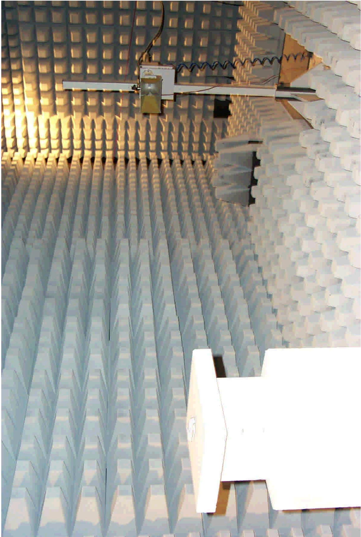
40451emi13.jpg: Test set-up preliminary radiated emission measurement
