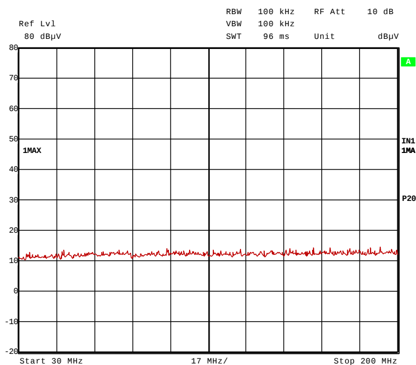
30448tx3a.wmf: 30 MHz to 200 MHz, transmit mode
