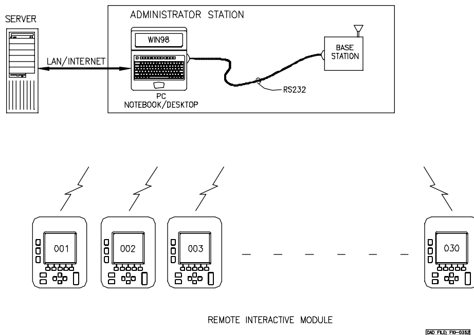
Figure 1. RSS Operation
