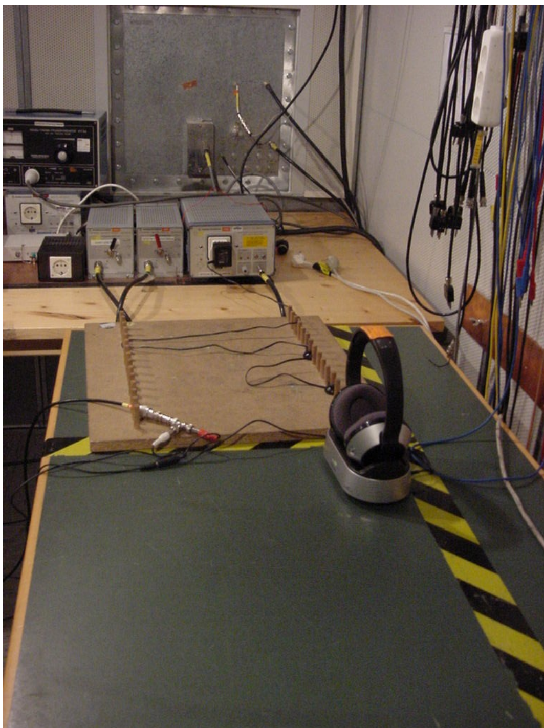
Photo 6 (Conducted Emissions): Charging mode
