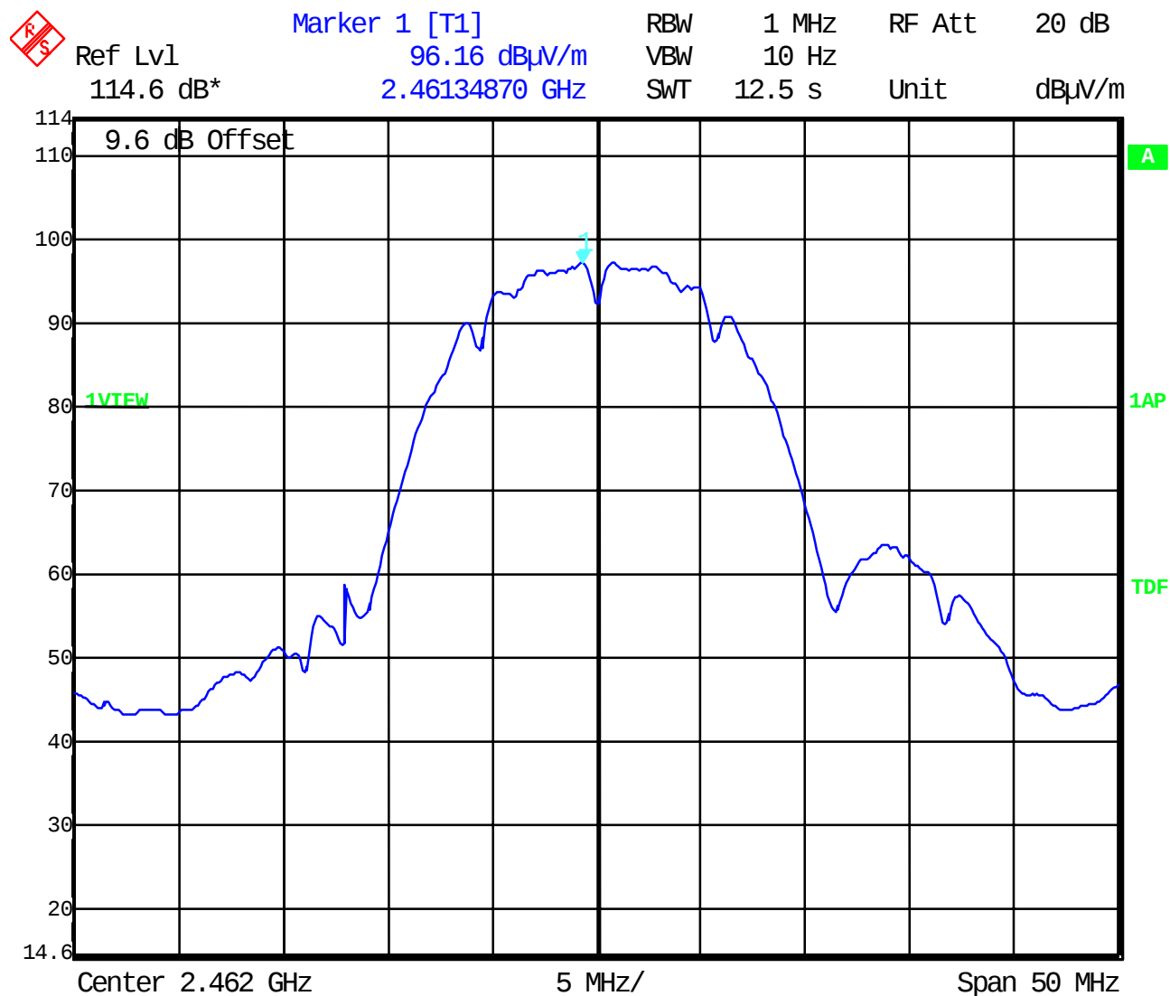
Plot 2 : Max field strength in 3m distance (single frequency) average
