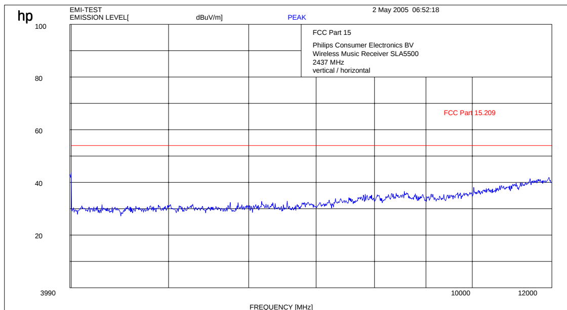
Plot 5: 4- 12 GHz (middle channel)
