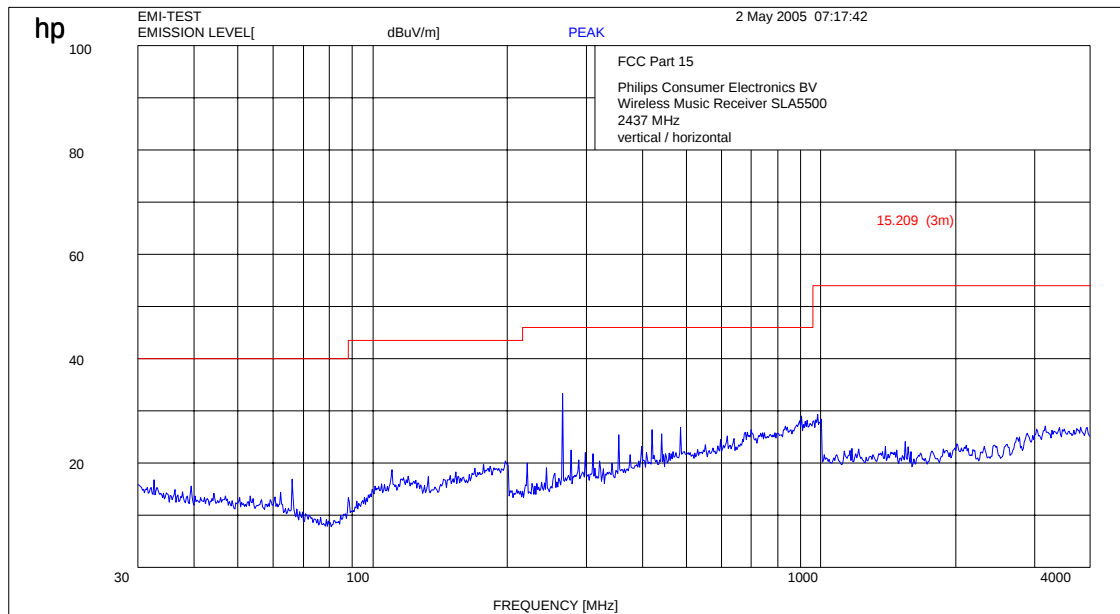
Plot 4: 0.03 - 4 GHz vertical / horizontal (middle channel)
