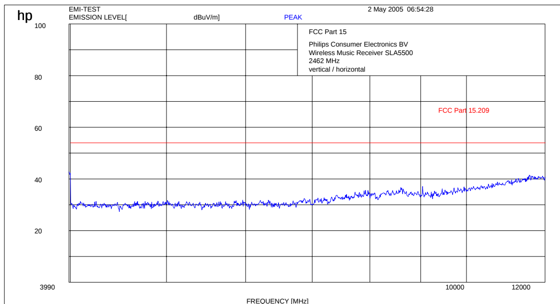
Carrier suppressed with a tunable filter to avoid overload of the preamp Plot 7: 4- 12 GHz (highest channel)
