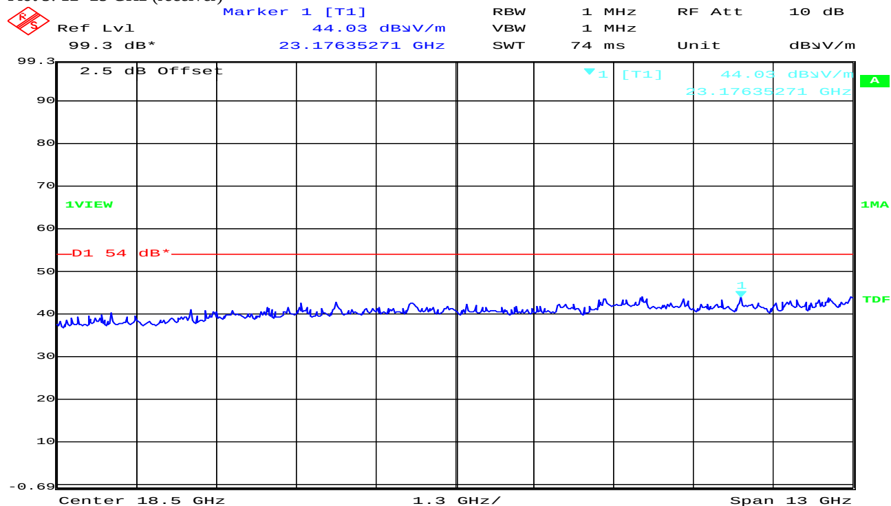
Plot 3: 12- 25 GHz (receiver)
